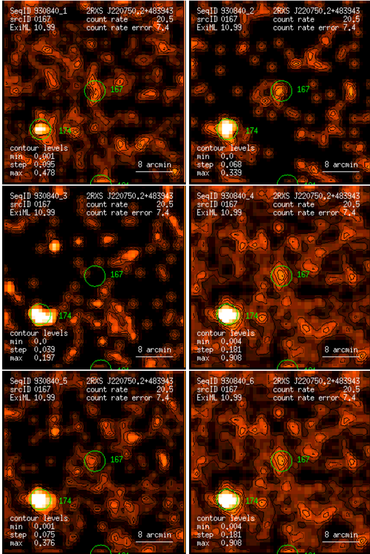
Figure 167: RASS 930840: detection 0167: band rate images, Gaussian filter: (1) PSPC channels 11 – 41, (2) 52 – 90, (3) 91 – 201, (4) 11 – 235, (5) 52 – 201, (6) 11 – 201. Broad band rates in counts/ks. Band rate contour levels in counts/ks/arcmin 2 .
