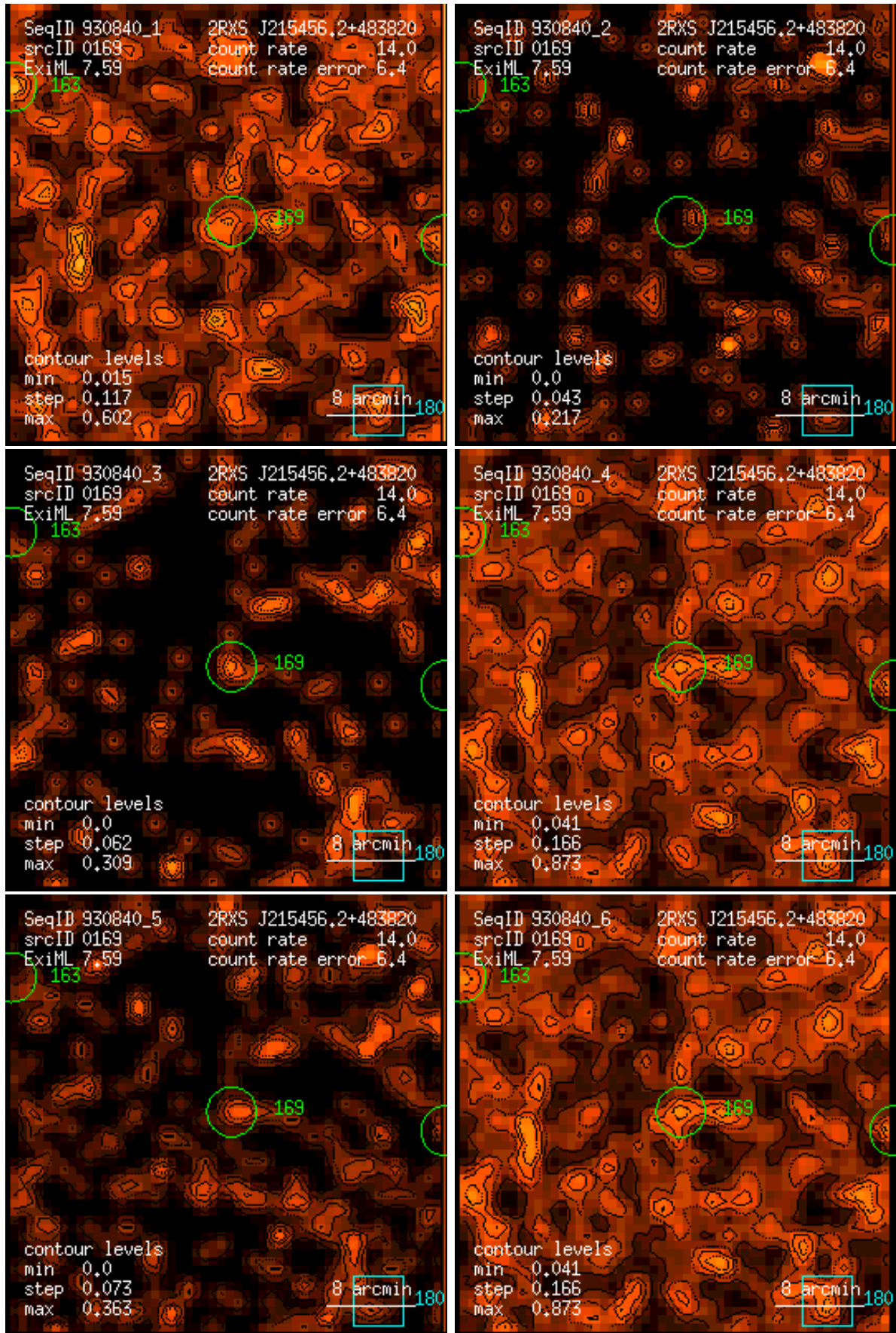
Figure 169: RASS 930840: detection 0169: band rate images, Gaussian filter: (1) PSPC channels 11 – 41, (2) 52 – 90, (3) 91 – 201, (4) 11 – 235, (5) 52 – 201, (6) 11 – 201. Broad band rates in counts/ks. Band rate contour levels in counts/ks/arcmin 2 .
