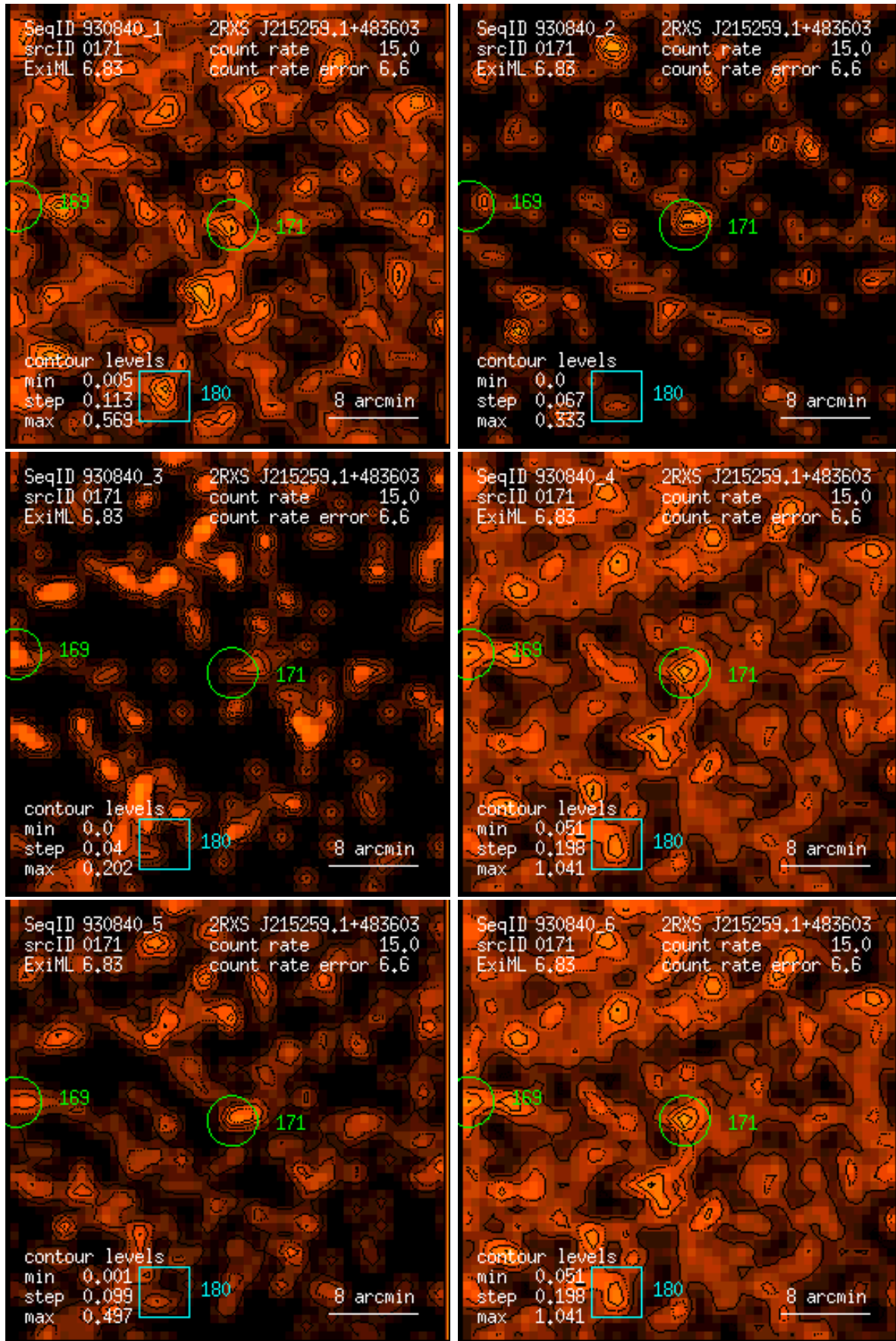
Figure 171: RASS 930840: detection 0171: band rate images, Gaussian filter: (1) PSPC channels 11 – 41, (2) 52 – 90, (3) 91 – 201, (4) 11 – 235, (5) 52 – 201, (6) 11 – 201. Broad band rates in counts/ks. Band rate contour levels in counts/ks/arcmin 2 .
