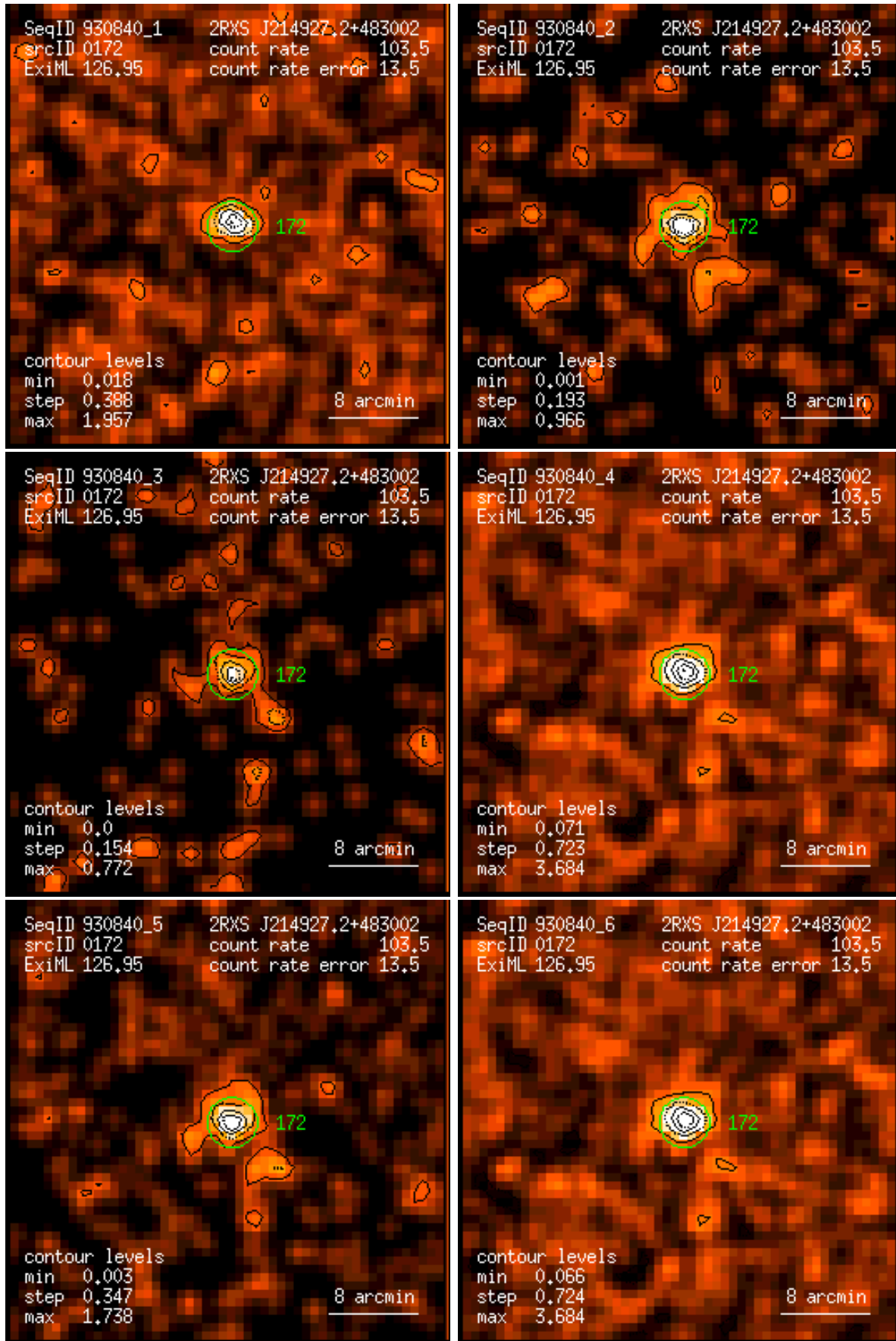
Figure 172: RASS 930840: detection 0172: band rate images, Gaussian filter: (1) PSPC channels 11 – 41, (2) 52 – 90, (3) 91 – 201, (4) 11 – 235, (5) 52 – 201, (6) 11 – 201. Broad band rates in counts/ks. Band rate contour levels in counts/ks/arcmin 2 .
