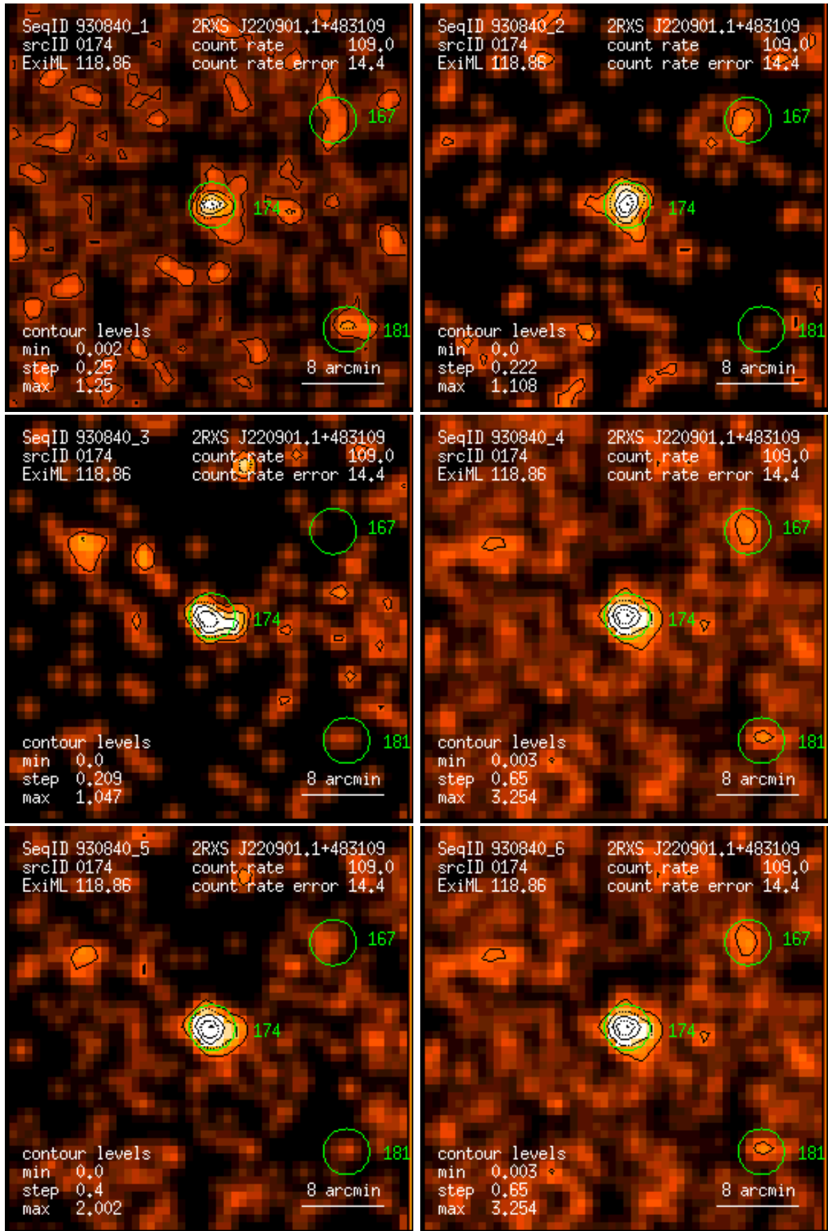
Figure 174: RASS 930840: detection 0174: band rate images, Gaussian filter: (1) PSPC channels 11 – 41, (2) 52 – 90, (3) 91 – 201, (4) 11 – 235, (5) 52 – 201, (6) 11 – 201. Broad band rates in counts/ks. Band rate contour levels in counts/ks/arcmin 2 .
