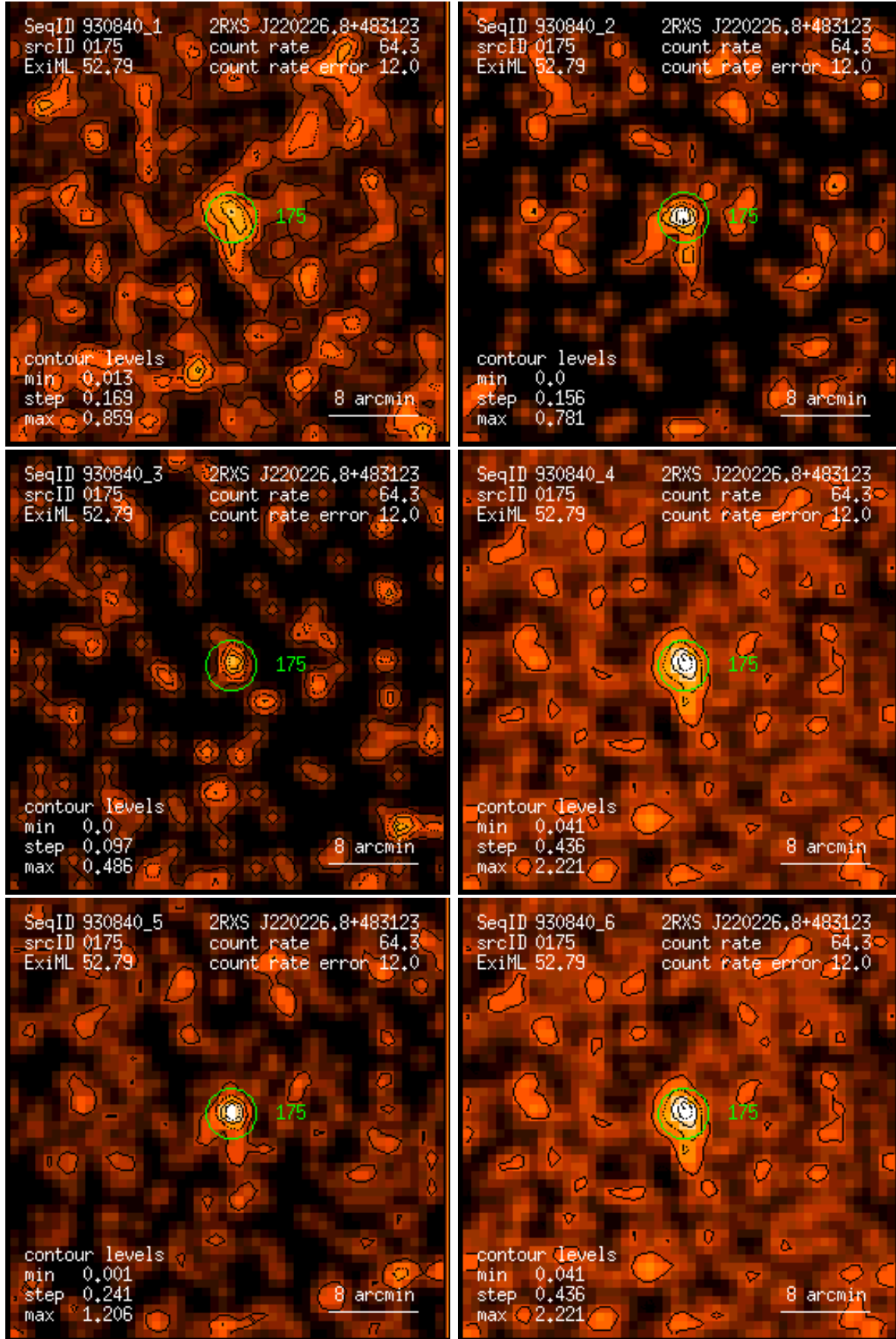
Figure 175: RASS 930840: detection 0175: band rate images, Gaussian filter: (1) PSPC channels 11 – 41, (2) 52 – 90, (3) 91 – 201, (4) 11 – 235, (5) 52 – 201, (6) 11 – 201. Broad band rates in counts/ks. Band rate contour levels in counts/ks/arcmin 2 .
