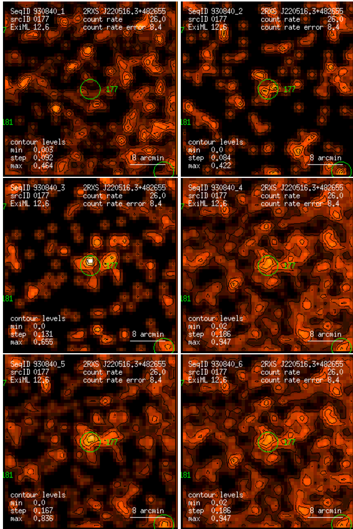
Figure 177: RASS 930840: detection 0177: band rate images, Gaussian filter: (1) PSPC channels 11 – 41, (2) 52 – 90, (3) 91 – 201, (4) 11 – 235, (5) 52 – 201, (6) 11 – 201. Broad band rates in counts/ks. Band rate contour levels in counts/ks/arcmin 2 .
