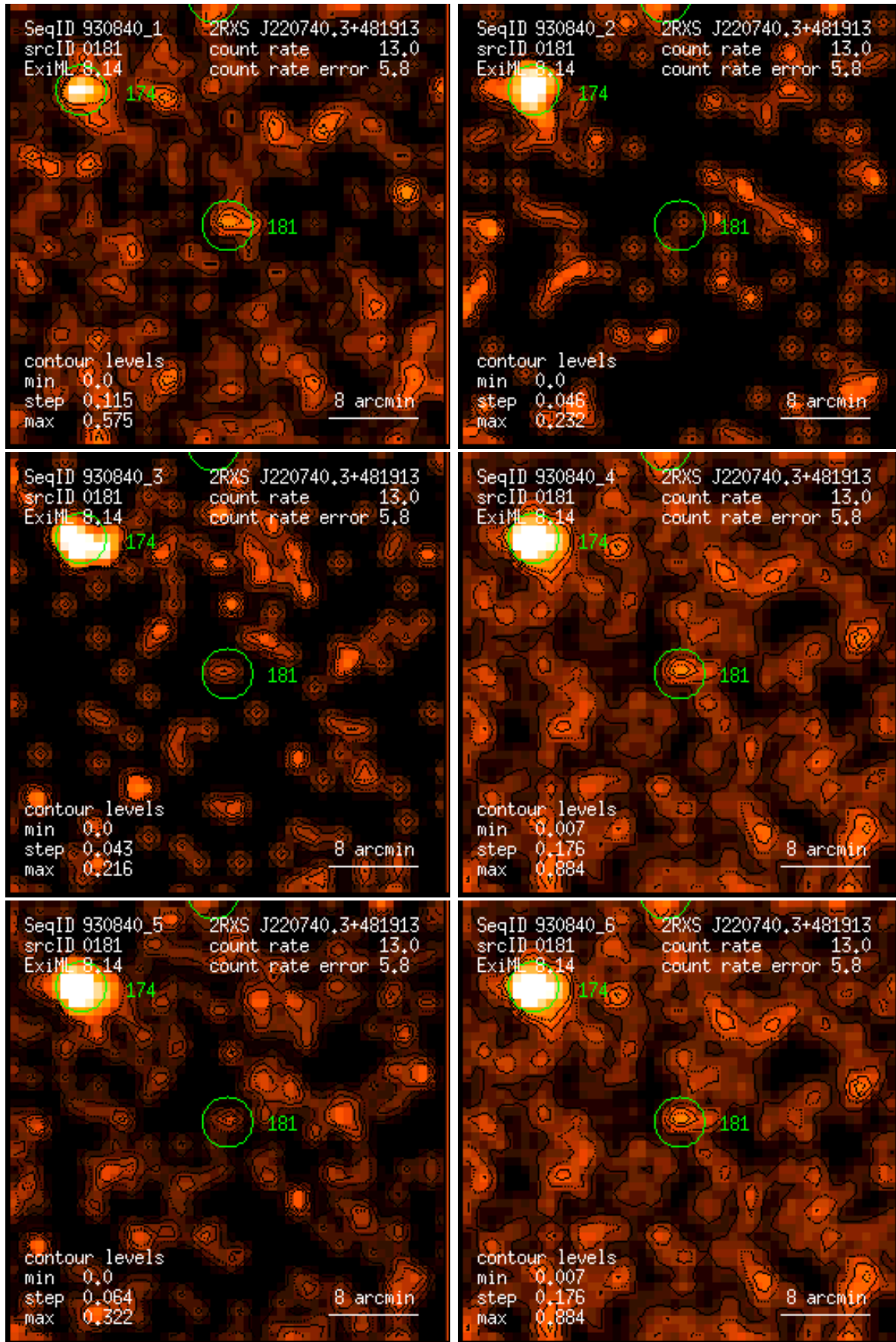
Figure 181: RASS 930840: detection 0181: band rate images, Gaussian filter: (1) PSPC channels 11 – 41, (2) 52 – 90, (3) 91 – 201, (4) 11 – 235, (5) 52 – 201, (6) 11 – 201. Broad band rates in counts/ks. Band rate contour levels in counts/ks/arcmin 2 .
