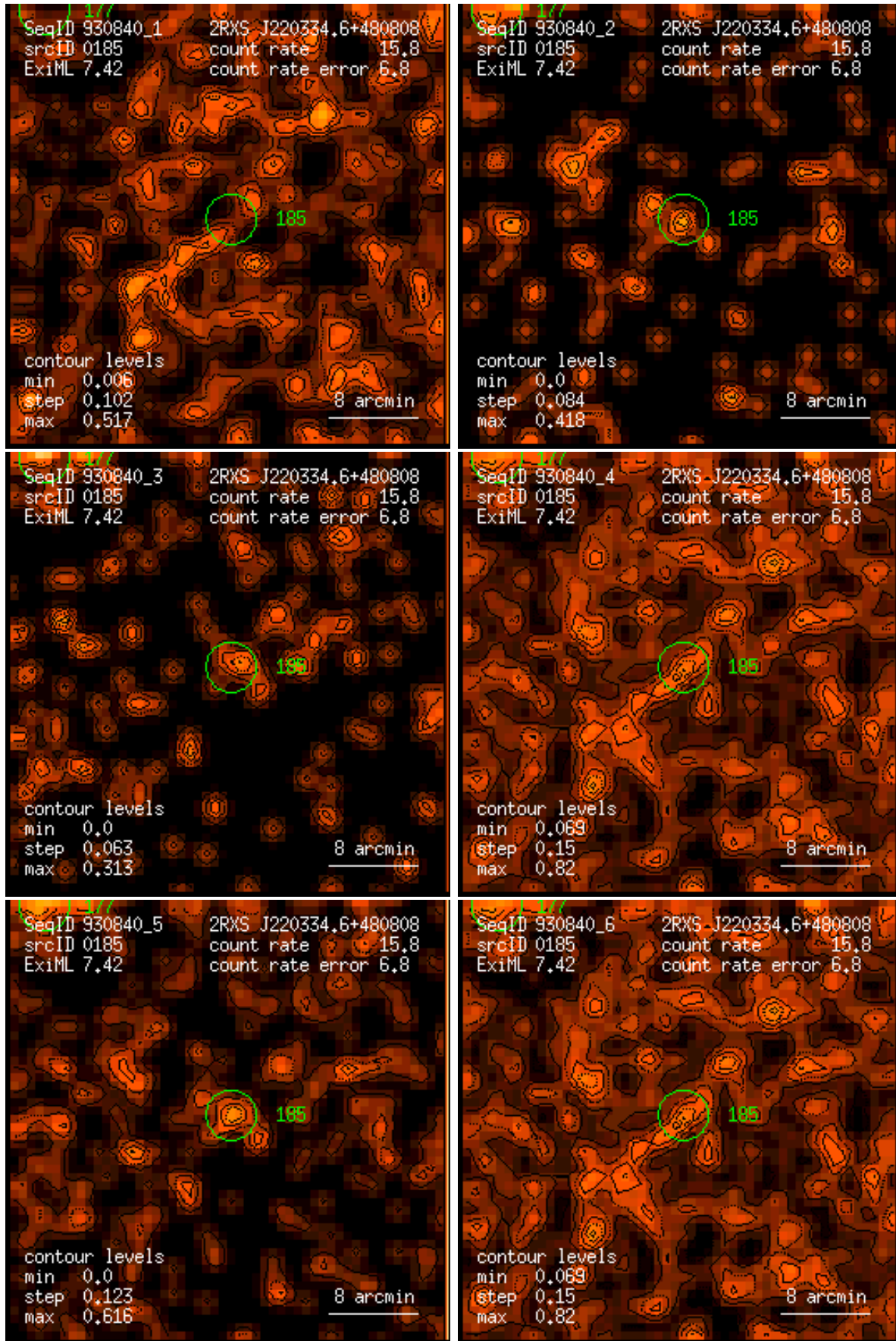
Figure 185: RASS 930840: detection 0185: band rate images, Gaussian filter: (1) PSPC channels 11 – 41, (2) 52 – 90, (3) 91 – 201, (4) 11 – 235, (5) 52 – 201, (6) 11 – 201. Broad band rates in counts/ks. Band rate contour levels in counts/ks/arcmin 2 .
