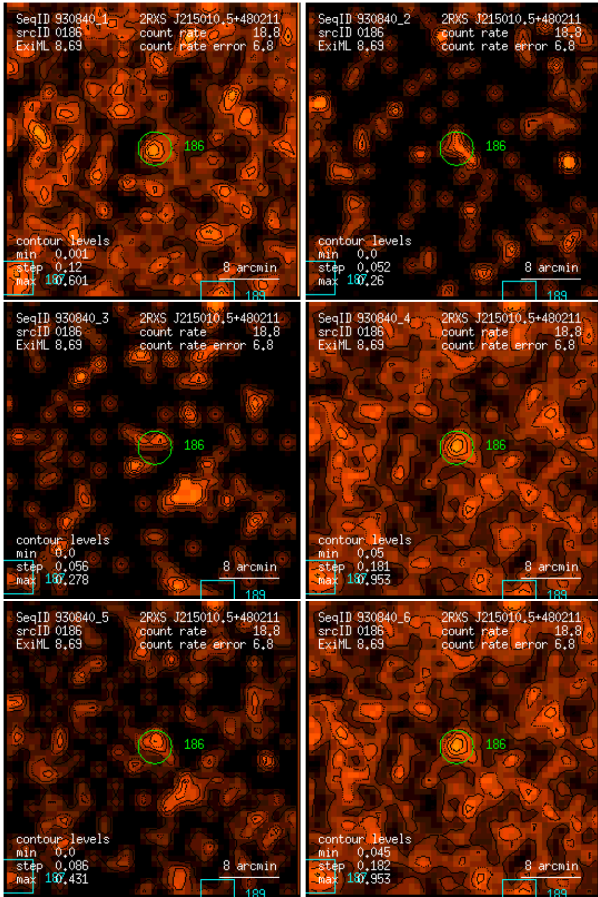
Figure 186: RASS 930840: detection 0186: band rate images, Gaussian filter: (1) PSPC channels 11 – 41, (2) 52 – 90, (3) 91 – 201, (4) 11 – 235, (5) 52 – 201, (6) 11 – 201. Broad band rates in counts/ks. Band rate contour levels in counts/ks/arcmin 2 .
