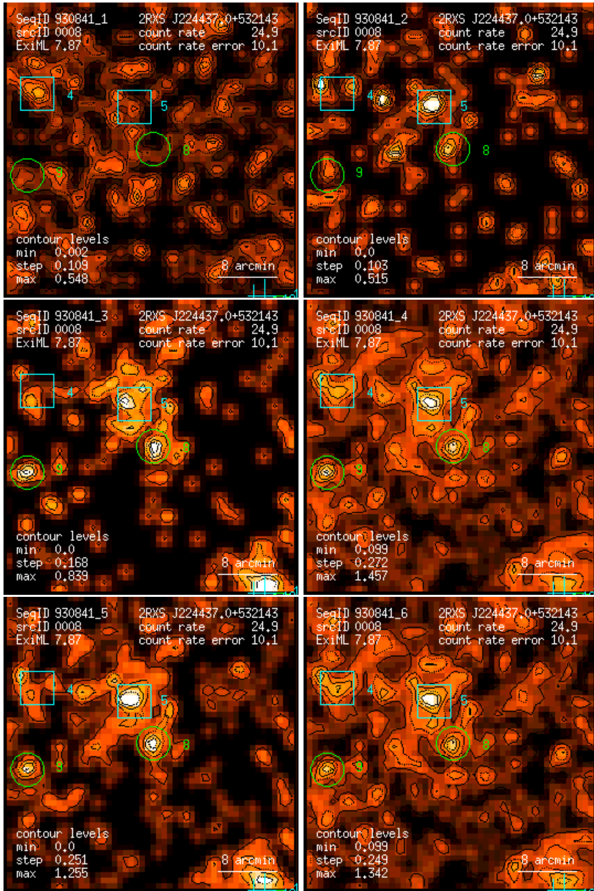
Figure 8: RASS 930841: detection 0008: band rate images, Gaussian filter: (1) PSPC channels 11 – 41, (2) 52 – 90, (3) 91 – 201, (4) 11 – 235, (5) 52 – 201, (6) 11 – 201. Broad band rates in counts/ks. Band rate contour levels in counts/ks/arcmin 2 .
