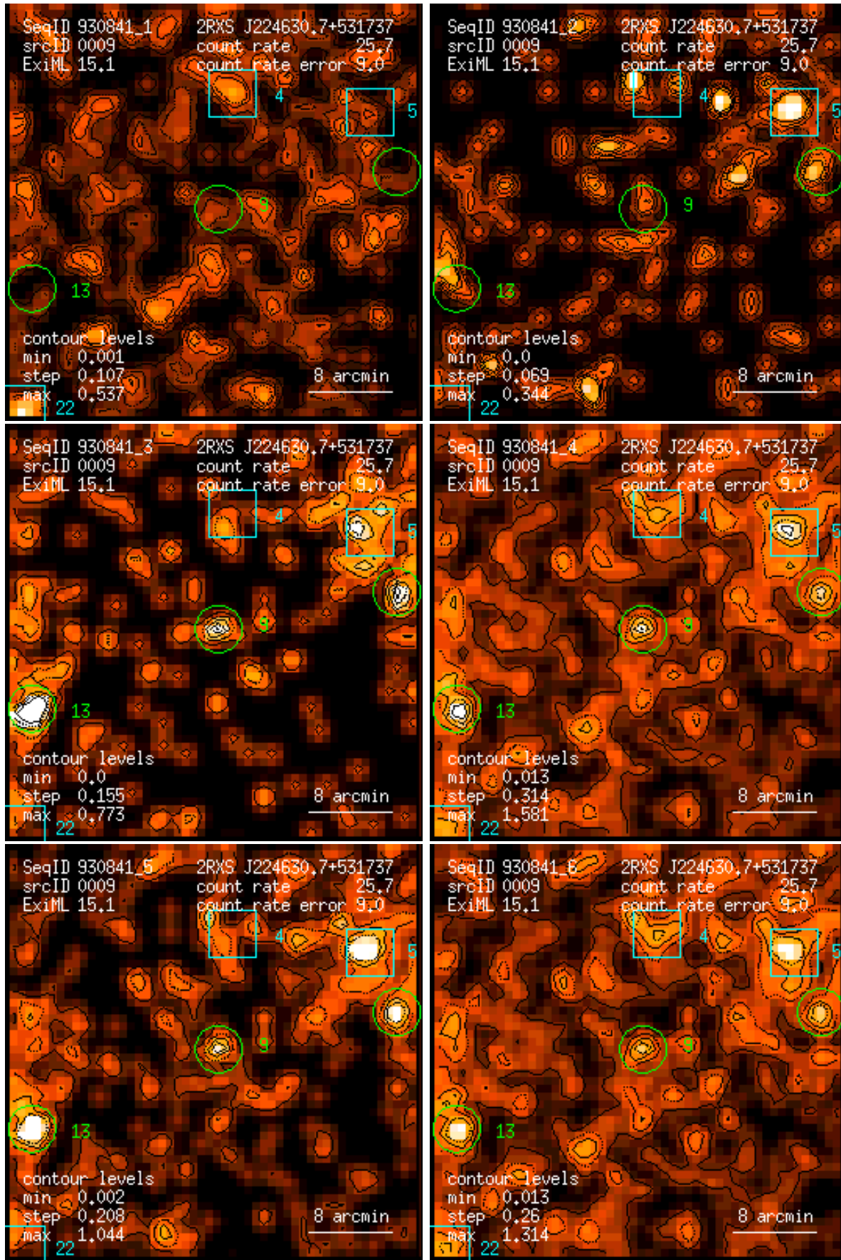
Figure 9: RASS 930841: detection 0009: band rate images, Gaussian filter: (1) PSPC channels 11 – 41, (2) 52 – 90, (3) 91 – 201, (4) 11 – 235, (5) 52 – 201, (6) 11 – 201. Broad band rates in counts/ks. Band rate contour levels in counts/ks/arcmin 2 .
