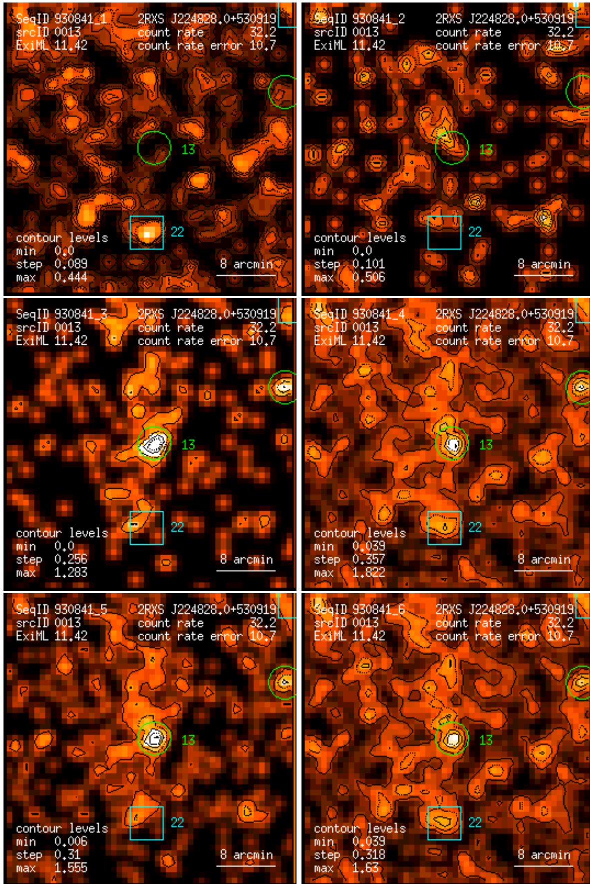
Figure 13: RASS 930841: detection 0013: band rate images, Gaussian filter: (1) PSPC channels 11 – 41, (2) 52 – 90, (3) 91 – 201, (4) 11 – 235, (5) 52 – 201, (6) 11 – 201. Broad band rates in counts/ks. Band rate contour levels in counts/ks/arcmin 2 .
