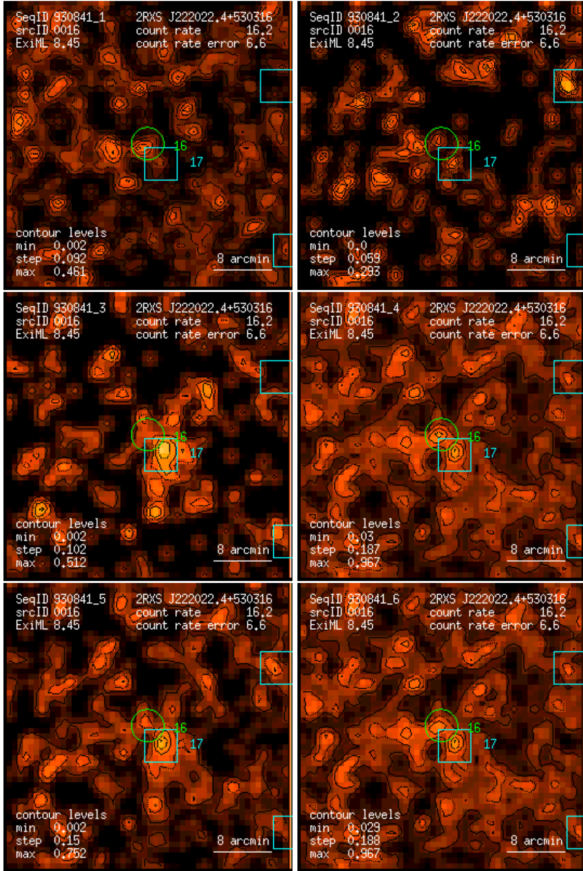
Figure 16: RASS 930841: detection 0016: band rate images, Gaussian filter: (1) PSPC channels 11 – 41, (2) 52 – 90, (3) 91 – 201, (4) 11 – 235, (5) 52 – 201, (6) 11 – 201. Broad band rates in counts/ks. Band rate contour levels in counts/ks/arcmin 2 .
