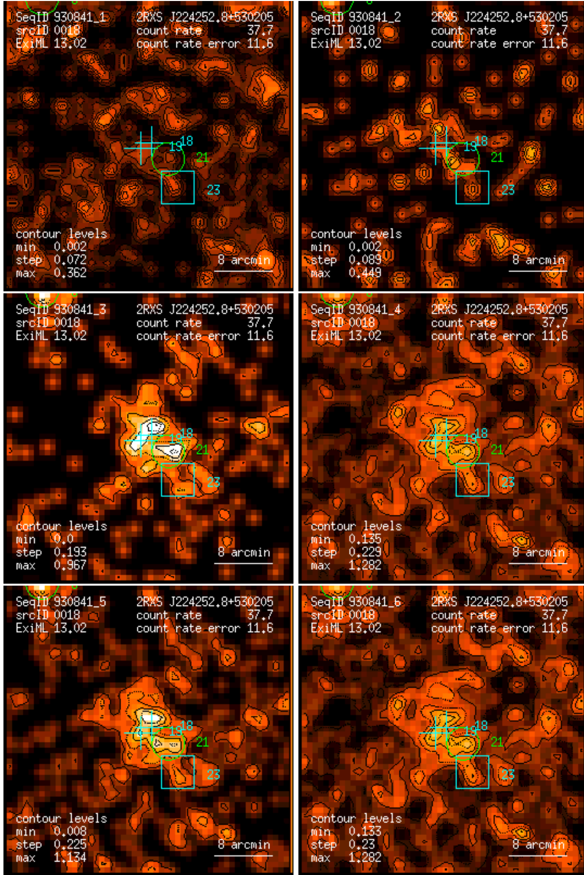
Figure 18: RASS 930841: detection 0018: band rate images, Gaussian filter: (1) PSPC channels 11 – 41, (2) 52 – 90, (3) 91 – 201, (4) 11 – 235, (5) 52 – 201, (6) 11 – 201. Broad band rates in counts/ks. Band rate contour levels in counts/ks/arcmin 2 .
