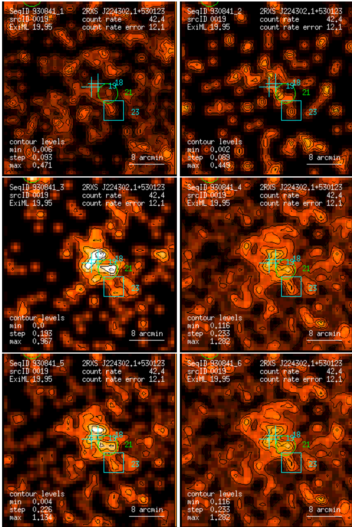
Figure 19: RASS 930841: detection 0019: band rate images, Gaussian filter: (1) PSPC channels 11 – 41, (2) 52 – 90, (3) 91 – 201, (4) 11 – 235, (5) 52 – 201, (6) 11 – 201. Broad band rates in counts/ks. Band rate contour levels in counts/ks/arcmin 2 .
