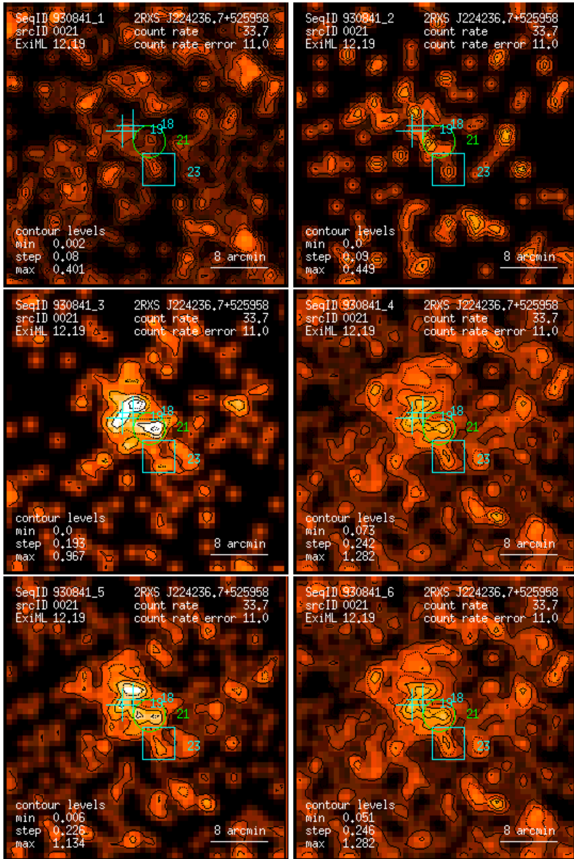
Figure 21: RASS 930841: detection 0021: band rate images, Gaussian filter: (1) PSPC channels 11 – 41, (2) 52 – 90, (3) 91 – 201, (4) 11 – 235, (5) 52 – 201, (6) 11 – 201. Broad band rates in counts/ks. Band rate contour levels in counts/ks/arcmin 2 .
