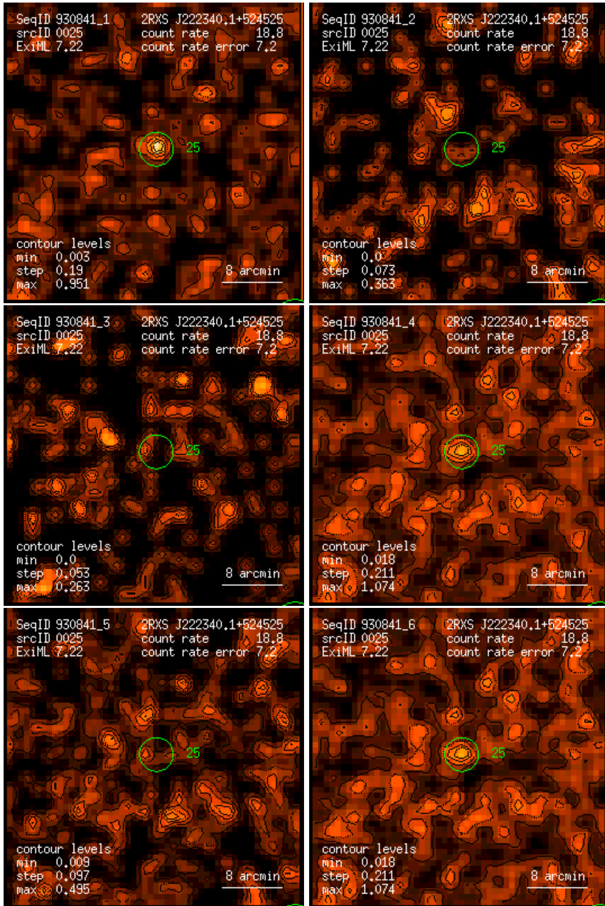
Figure 25: RASS 930841: detection 0025: band rate images, Gaussian filter: (1) PSPC channels 11 – 41, (2) 52 – 90, (3) 91 – 201, (4) 11 – 235, (5) 52 – 201, (6) 11 – 201. Broad band rates in counts/ks. Band rate contour levels in counts/ks/arcmin 2 .
