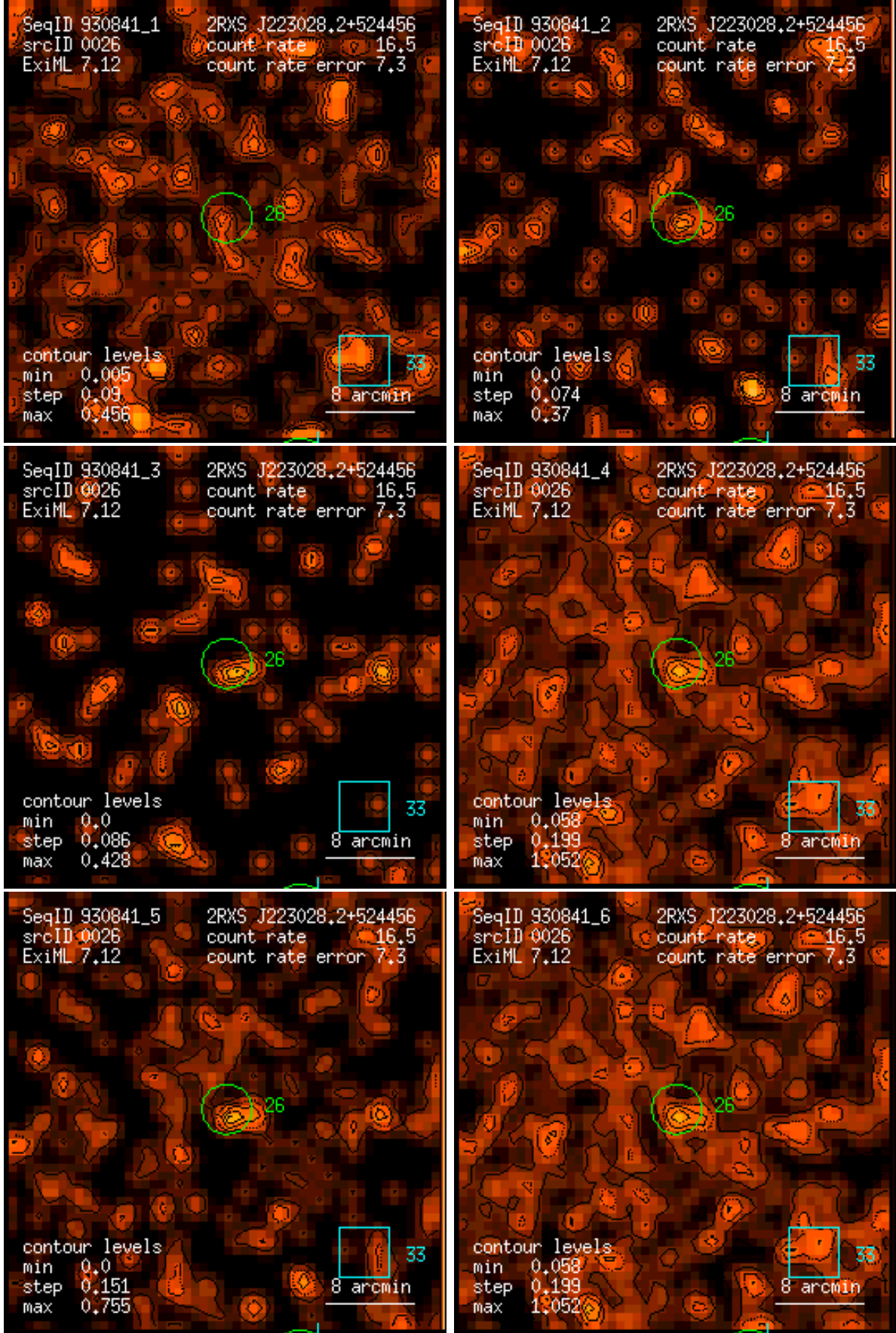
Figure 26: RASS 930841: detection 0026: band rate images, Gaussian filter: (1) PSPC channels 11 – 41, (2) 52 – 90, (3) 91 – 201, (4) 11 – 235, (5) 52 – 201, (6) 11 – 201. Broad band rates in counts/ks. Band rate contour levels in counts/ks/arcmin 2 .
