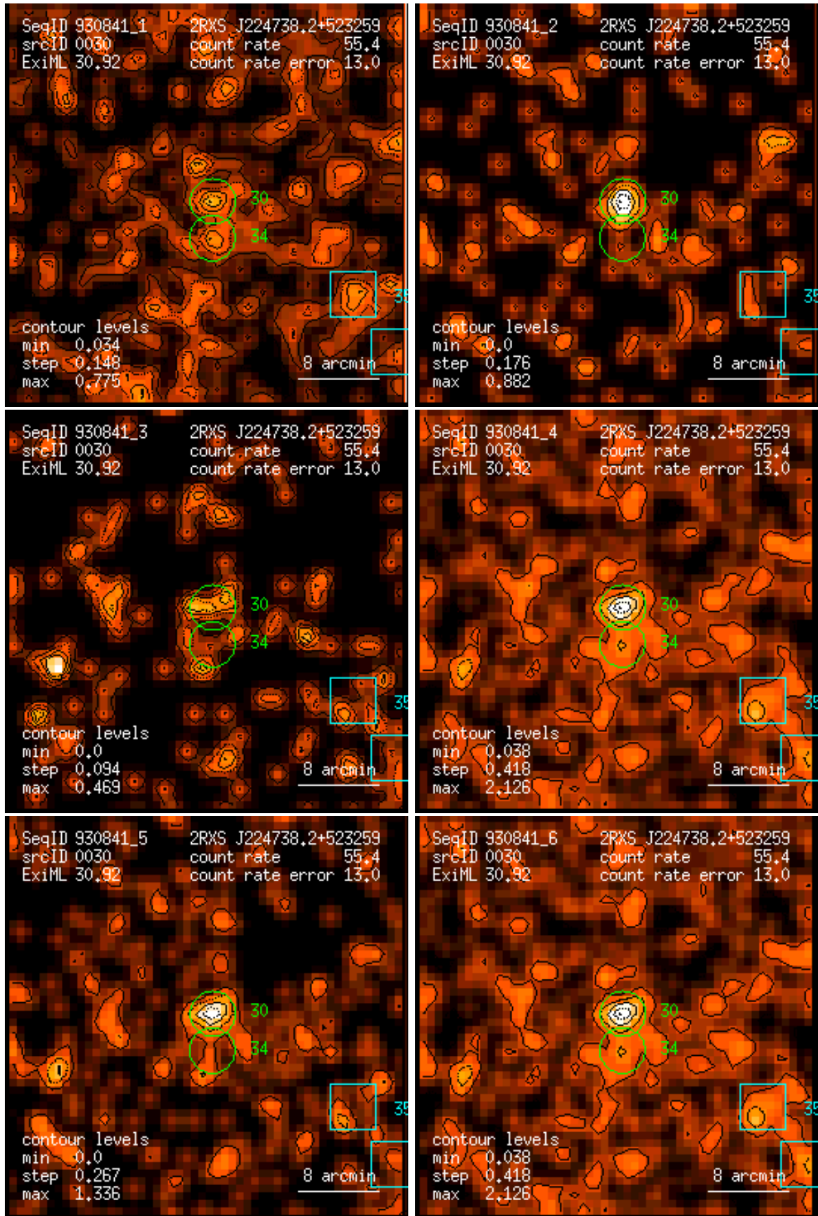
Figure 30: RASS 930841: detection 0030: band rate images, Gaussian filter: (1) PSPC channels 11 – 41, (2) 52 – 90, (3) 91 – 201, (4) 11 – 235, (5) 52 – 201, (6) 11 – 201. Broad band rates in counts/ks. Band rate contour levels in counts/ks/arcmin 2 .
