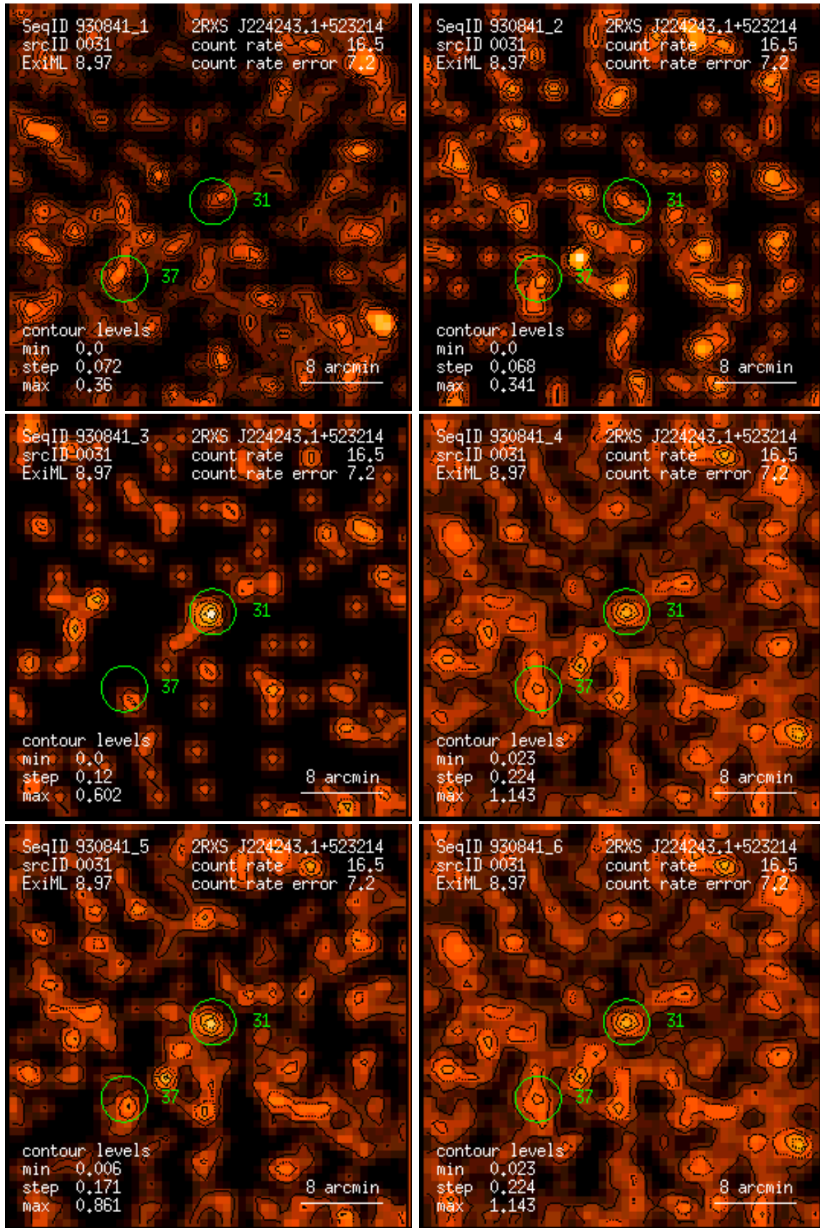
Figure 31: RASS 930841: detection 0031: band rate images, Gaussian filter: (1) PSPC channels 11 – 41, (2) 52 – 90, (3) 91 – 201, (4) 11 – 235, (5) 52 – 201, (6) 11 – 201. Broad band rates in counts/ks. Band rate contour levels in counts/ks/arcmin 2 .
