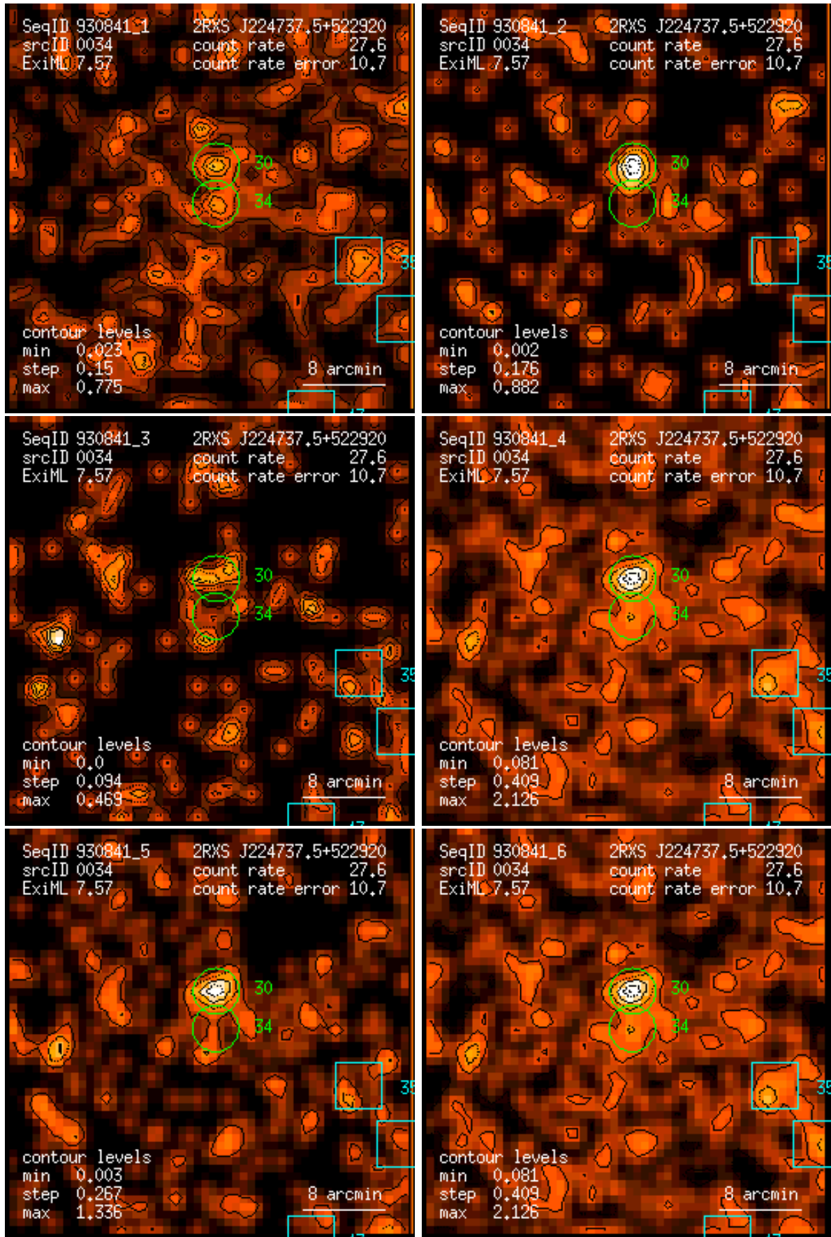
Figure 34: RASS 930841: detection 0034: band rate images, Gaussian filter: (1) PSPC channels 11 – 41, (2) 52 – 90, (3) 91 – 201, (4) 11 – 235, (5) 52 – 201, (6) 11 – 201. Broad band rates in counts/ks. Band rate contour levels in counts/ks/arcmin 2 .
