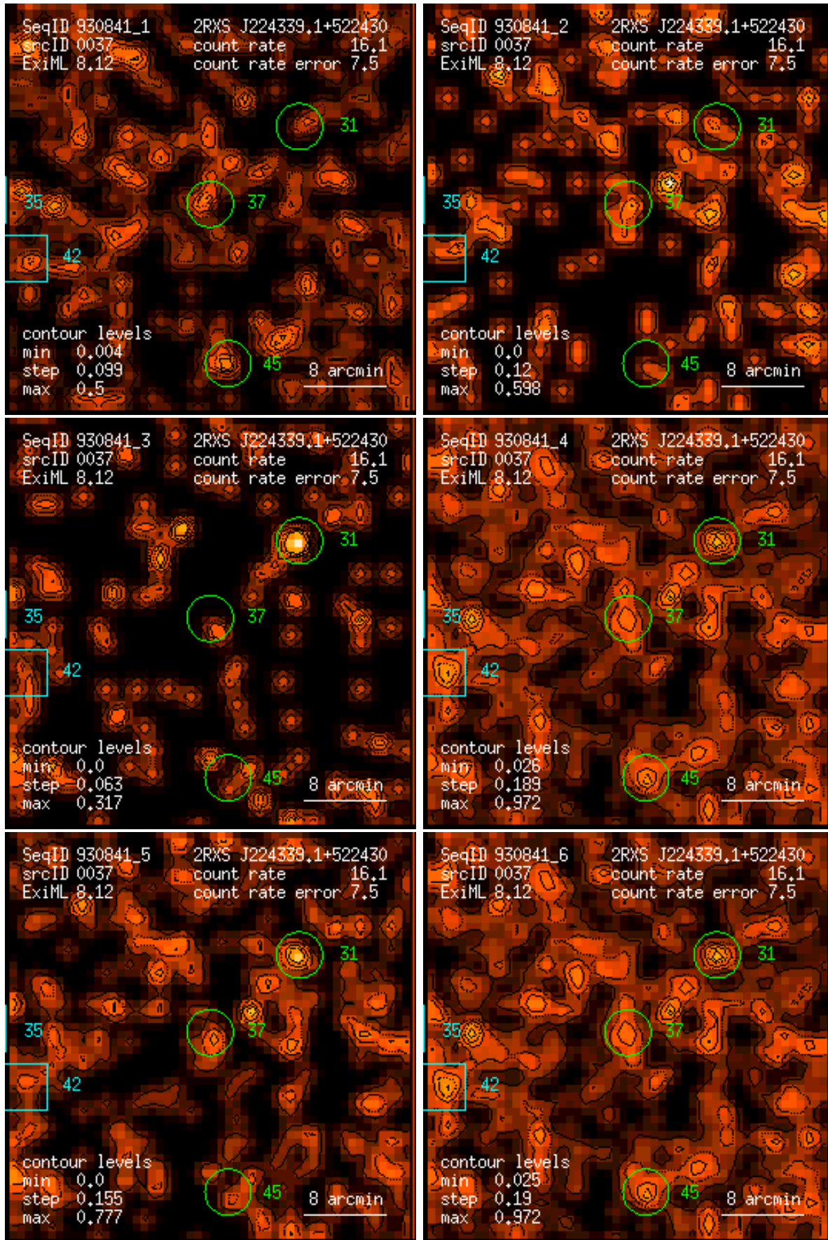
Figure 37: RASS 930841: detection 0037: band rate images, Gaussian filter: (1) PSPC channels 11 – 41, (2) 52 – 90, (3) 91 – 201, (4) 11 – 235, (5) 52 – 201, (6) 11 – 201. Broad band rates in counts/ks. Band rate contour levels in counts/ks/arcmin 2 .
