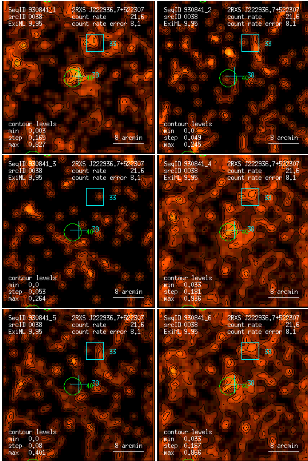
Figure 38: RASS 930841: detection 0038: band rate images, Gaussian filter: (1) PSPC channels 11 – 41, (2) 52 – 90, (3) 91 – 201, (4) 11 – 235, (5) 52 – 201, (6) 11 – 201. Broad band rates in counts/ks. Band rate contour levels in counts/ks/arcmin 2 .
