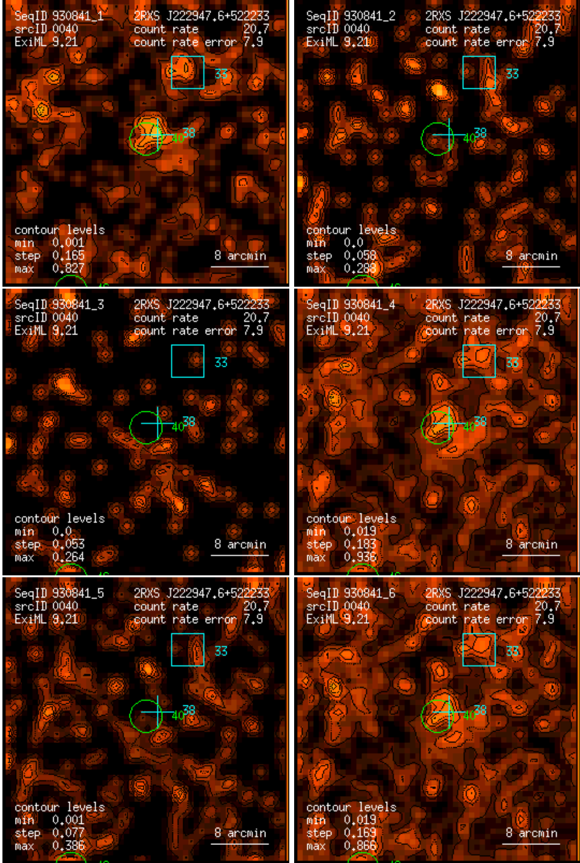
Figure 40: RASS 930841: detection 0040: band rate images, Gaussian filter: (1) PSPC channels 11 – 41, (2) 52 – 90, (3) 91 – 201, (4) 11 – 235, (5) 52 – 201, (6) 11 – 201. Broad band rates in counts/ks. Band rate contour levels in counts/ks/arcmin 2 .
