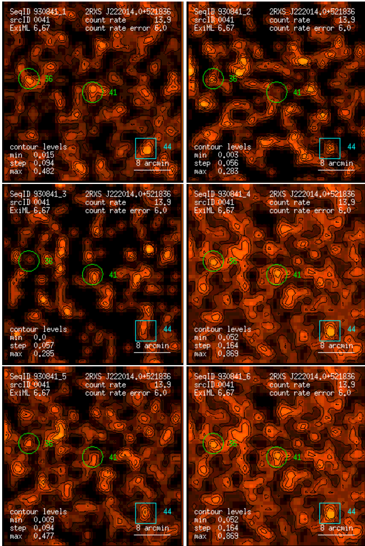
Figure 41: RASS 930841: detection 0041: band rate images, Gaussian filter: (1) PSPC channels 11 – 41, (2) 52 – 90, (3) 91 – 201, (4) 11 – 235, (5) 52 – 201, (6) 11 – 201. Broad band rates in counts/ks. Band rate contour levels in counts/ks/arcmin 2 .
