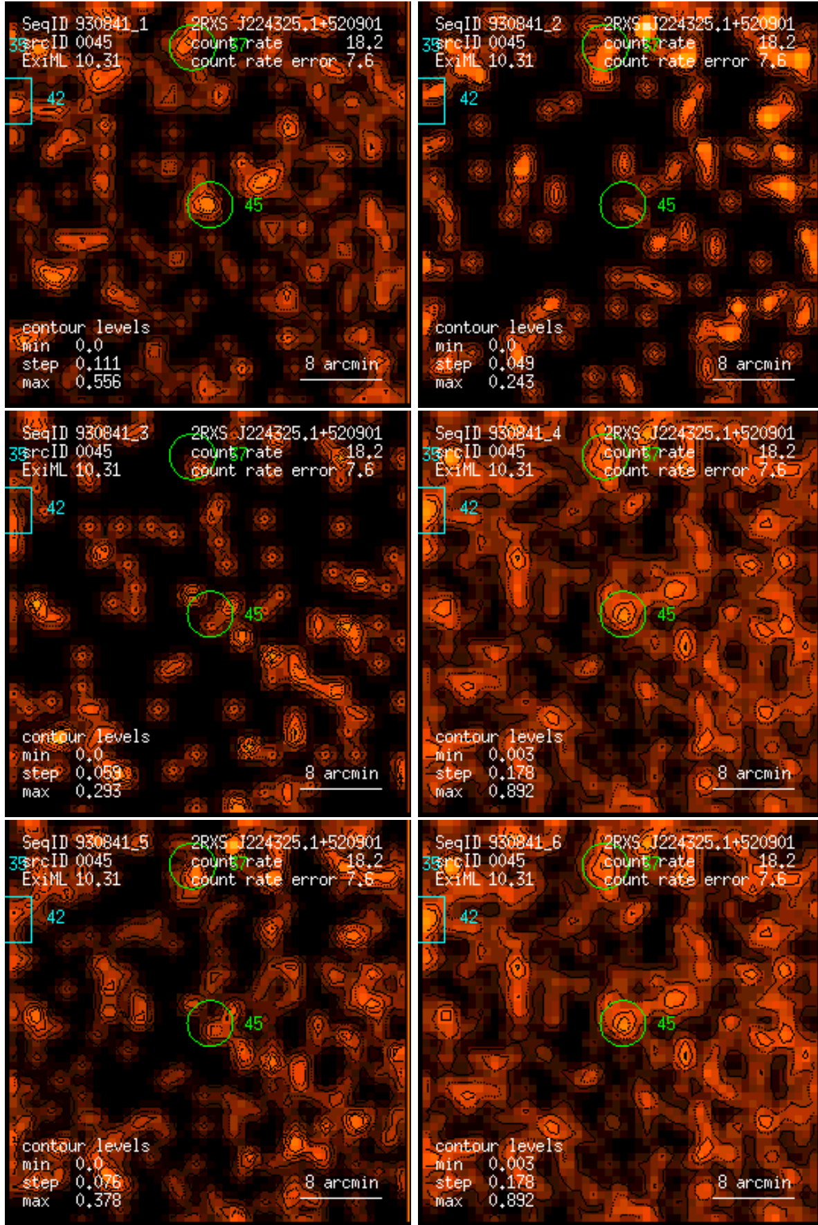
Figure 45: RASS 930841: detection 0045: band rate images, Gaussian filter: (1) PSPC channels 11 – 41, (2) 52 – 90, (3) 91 – 201, (4) 11 – 235, (5) 52 – 201, (6) 11 – 201. Broad band rates in counts/ks. Band rate contour levels in counts/ks/arcmin 2 .
