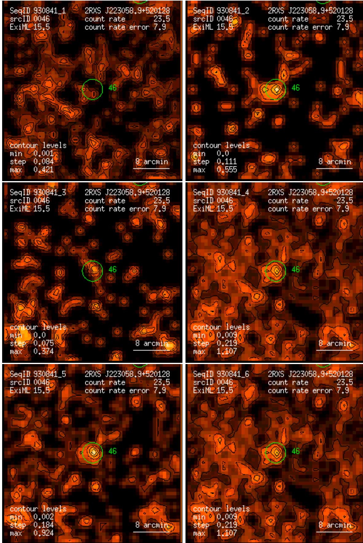
Figure 46: RASS 930841: detection 0046: band rate images, Gaussian filter: (1) PSPC channels 11 – 41, (2) 52 – 90, (3) 91 – 201, (4) 11 – 235, (5) 52 – 201, (6) 11 – 201. Broad band rates in counts/ks. Band rate contour levels in counts/ks/arcmin 2 .
