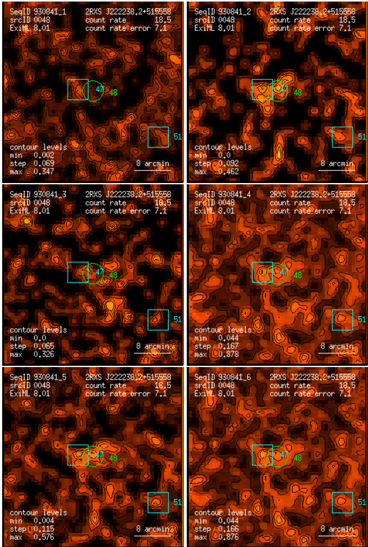
Figure 48: RASS 930841: detection 0048: band rate images, Gaussian filter: (1) PSPC channels 11 – 41, (2) 52 – 90, (3) 91 – 201, (4) 11 – 235, (5) 52 – 201, (6) 11 – 201. Broad band rates in counts/ks. Band rate contour levels in counts/ks/arcmin 2 .
