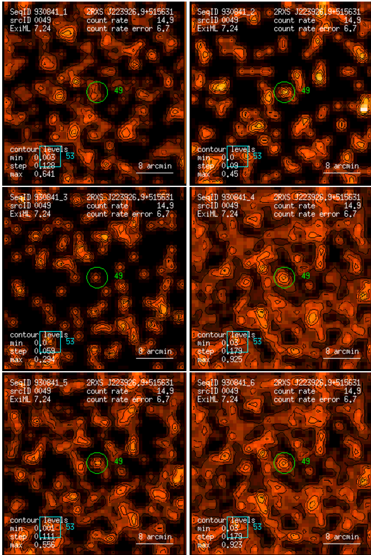
Figure 49: RASS 930841: detection 0049: band rate images, Gaussian filter: (1) PSPC channels 11 – 41, (2) 52 – 90, (3) 91 – 201, (4) 11 – 235, (5) 52 – 201, (6) 11 – 201. Broad band rates in counts/ks. Band rate contour levels in counts/ks/arcmin 2 .
