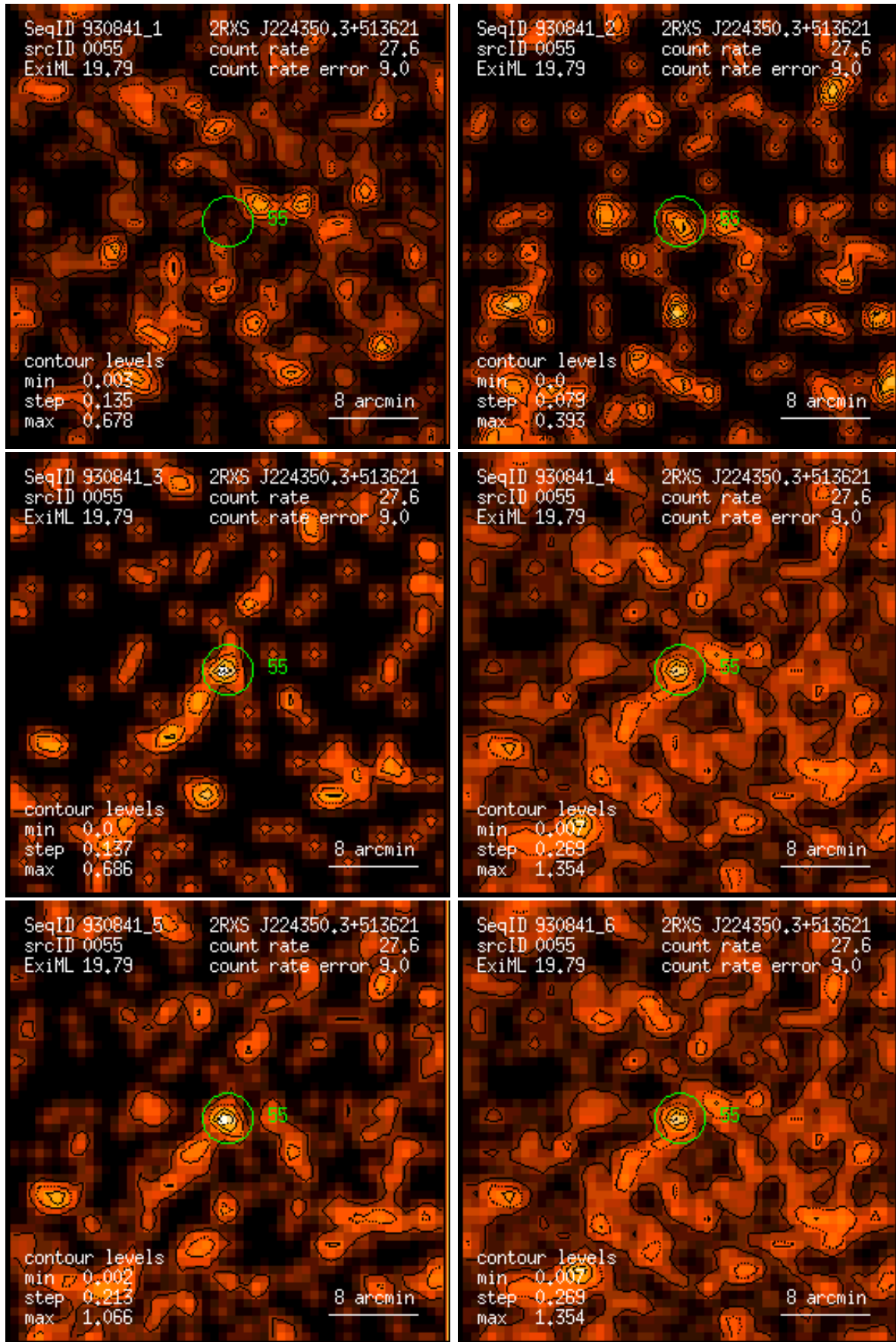
Figure 55: RASS 930841: detection 0055: band rate images, Gaussian filter: (1) PSPC channels 11 – 41, (2) 52 – 90, (3) 91 – 201, (4) 11 – 235, (5) 52 – 201, (6) 11 – 201. Broad band rates in counts/ks. Band rate contour levels in counts/ks/arcmin 2 .
