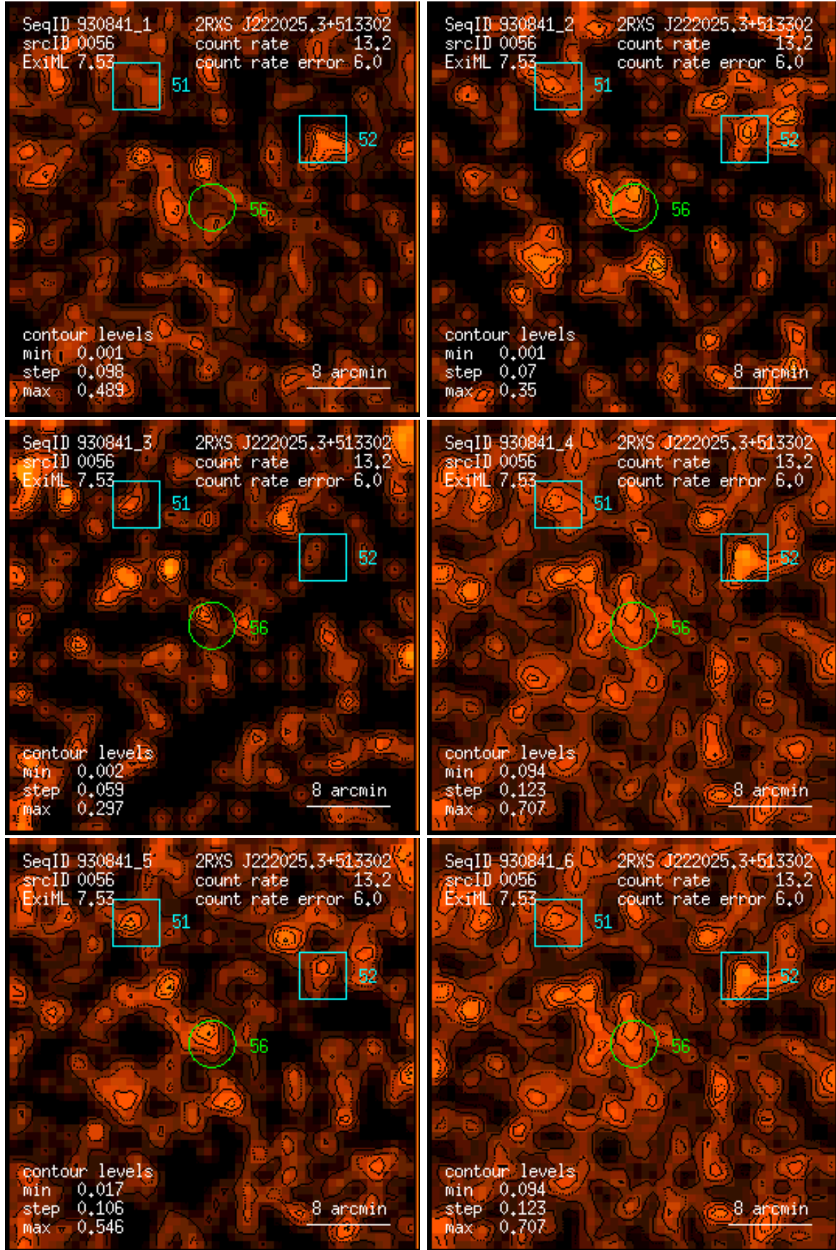
Figure 56: RASS 930841: detection 0056: band rate images, Gaussian filter: (1) PSPC channels 11 – 41, (2) 52 – 90, (3) 91 – 201, (4) 11 – 235, (5) 52 – 201, (6) 11 – 201. Broad band rates in counts/ks. Band rate contour levels in counts/ks/arcmin 2 .
