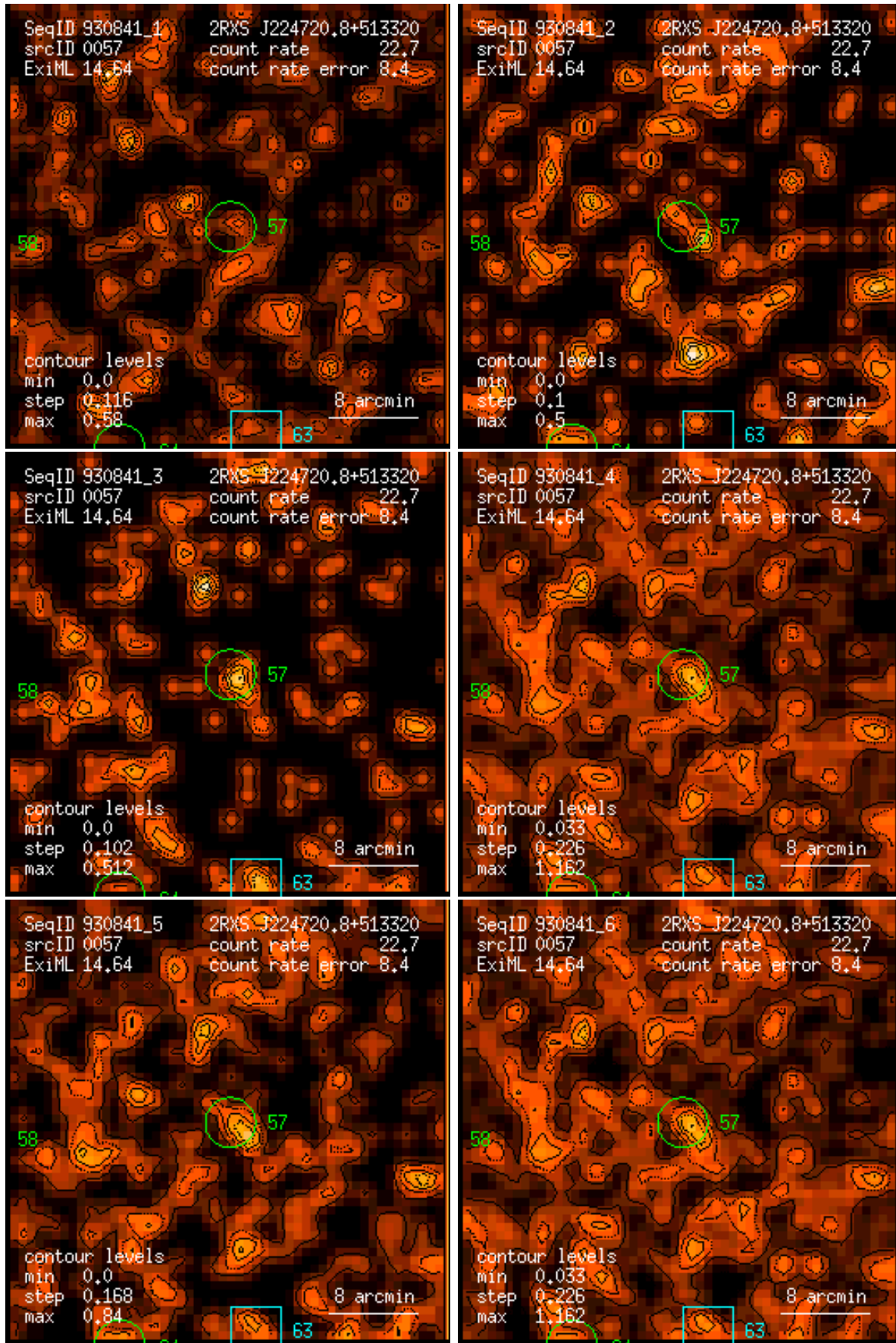
Figure 57: RASS 930841: detection 0057: band rate images, Gaussian filter: (1) PSPC channels 11 – 41, (2) 52 – 90, (3) 91 – 201, (4) 11 – 235, (5) 52 – 201, (6) 11 – 201. Broad band rates in counts/ks. Band rate contour levels in counts/ks/arcmin 2 .
