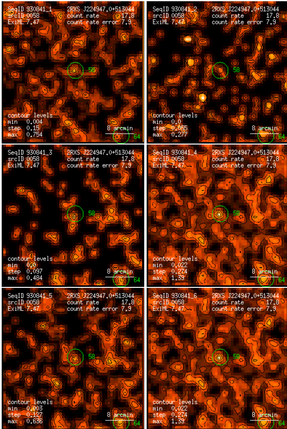
Figure 58: RASS 930841: detection 0058: band rate images, Gaussian filter: (1) PSPC channels 11 – 41, (2) 52 – 90, (3) 91 – 201, (4) 11 – 235, (5) 52 – 201, (6) 11 – 201. Broad band rates in counts/ks. Band rate contour levels in counts/ks/arcmin 2 .
