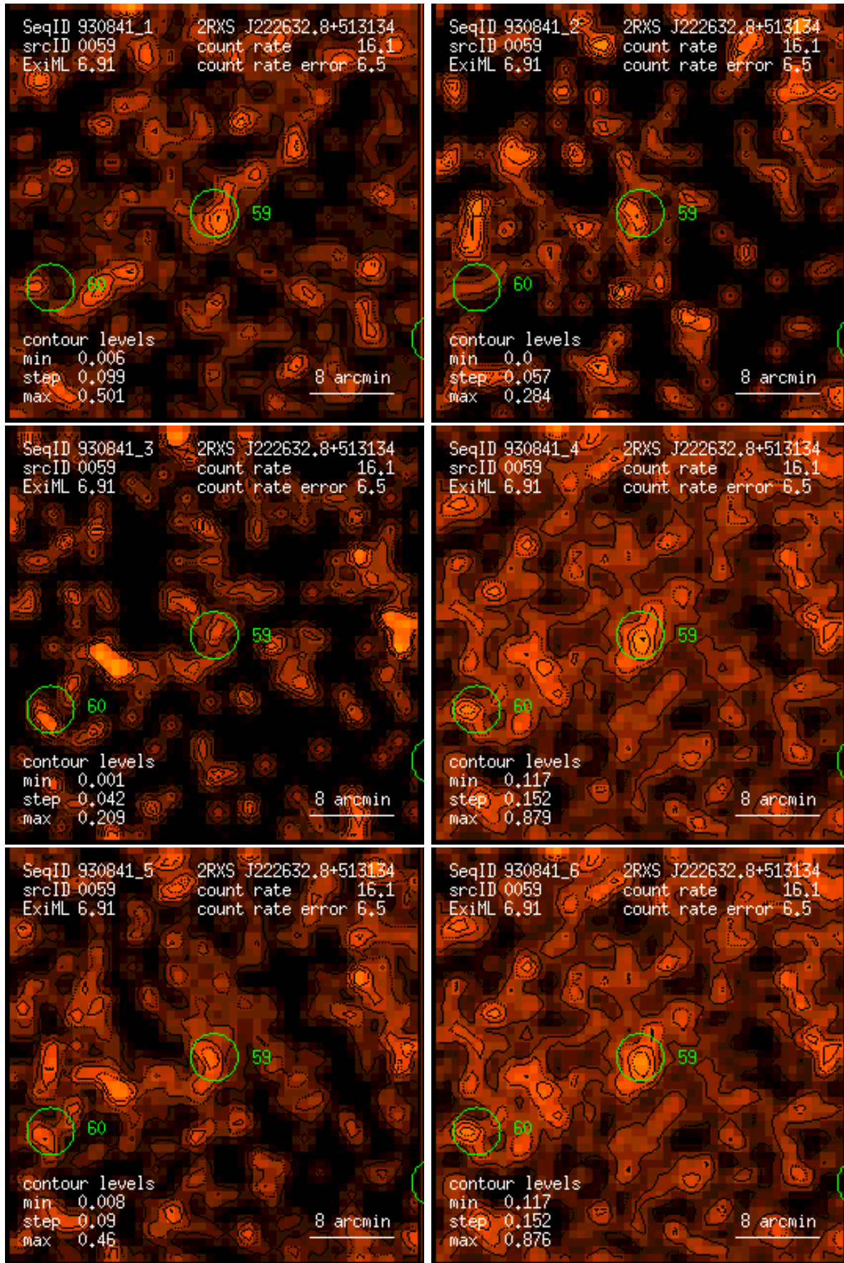
Figure 59: RASS 930841: detection 0059: band rate images, Gaussian filter: (1) PSPC channels 11 – 41, (2) 52 – 90, (3) 91 – 201, (4) 11 – 235, (5) 52 – 201, (6) 11 – 201. Broad band rates in counts/ks. Band rate contour levels in counts/ks/arcmin 2 .
