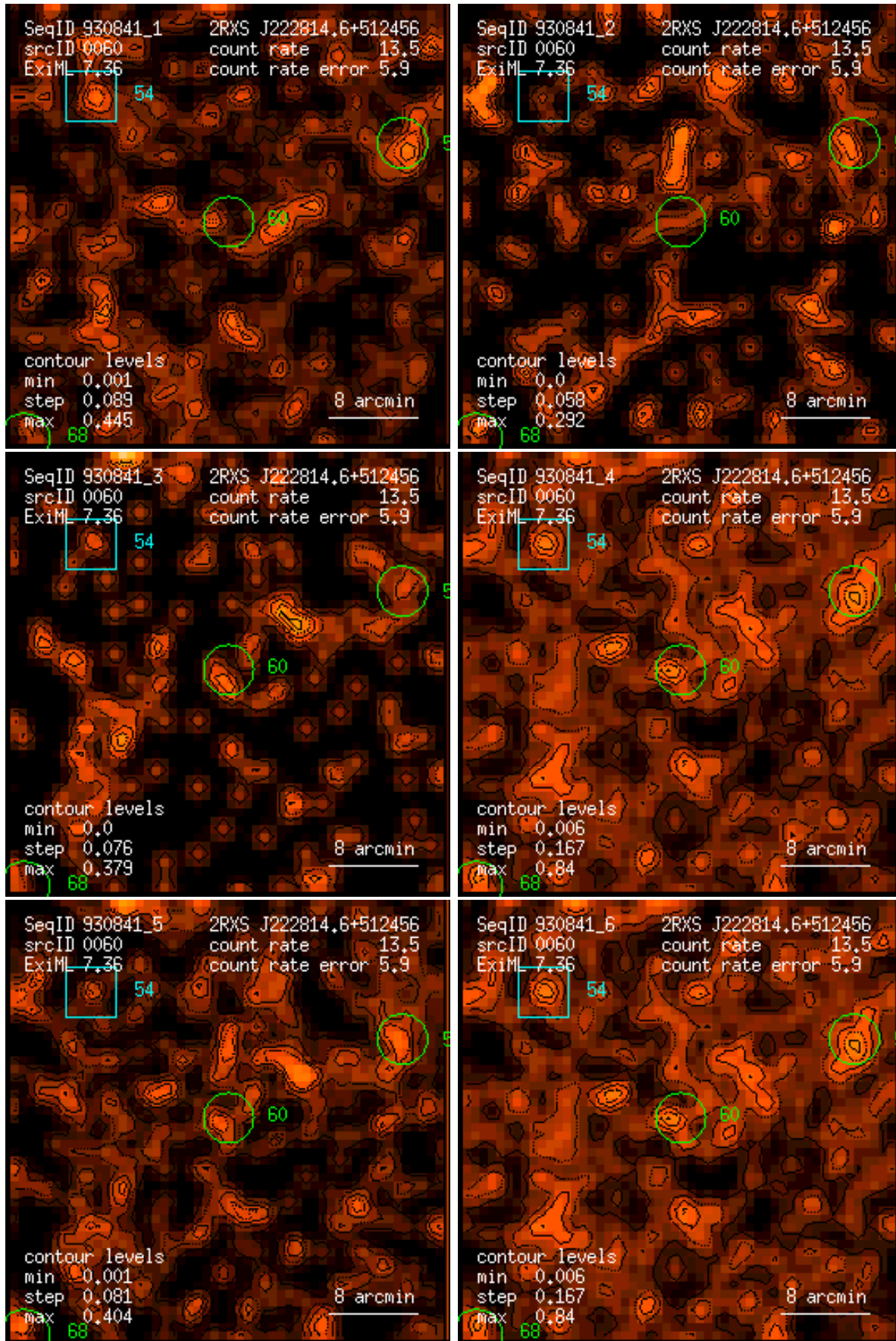
Figure 60: RASS 930841: detection 0060: band rate images, Gaussian filter: (1) PSPC channels 11 – 41, (2) 52 – 90, (3) 91 – 201, (4) 11 – 235, (5) 52 – 201, (6) 11 – 201. Broad band rates in counts/ks. Band rate contour levels in counts/ks/arcmin 2 .
