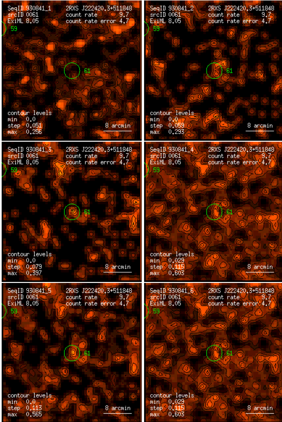
Figure 61: RASS 930841: detection 0061: band rate images, Gaussian filter: (1) PSPC channels 11 – 41, (2) 52 – 90, (3) 91 – 201, (4) 11 – 235, (5) 52 – 201, (6) 11 – 201. Broad band rates in counts/ks. Band rate contour levels in counts/ks/arcmin 2 .
