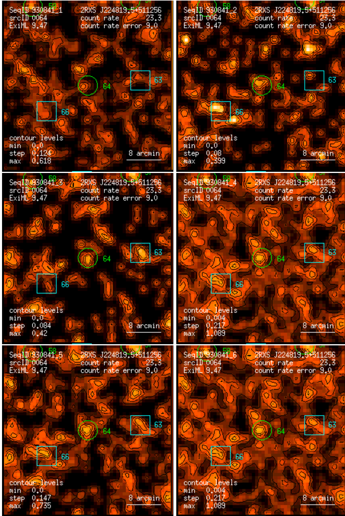
Figure 64: RASS 930841: detection 0064: band rate images, Gaussian filter: (1) PSPC channels 11 – 41, (2) 52 – 90, (3) 91 – 201, (4) 11 – 235, (5) 52 – 201, (6) 11 – 201. Broad band rates in counts/ks. Band rate contour levels in counts/ks/arcmin 2 .
