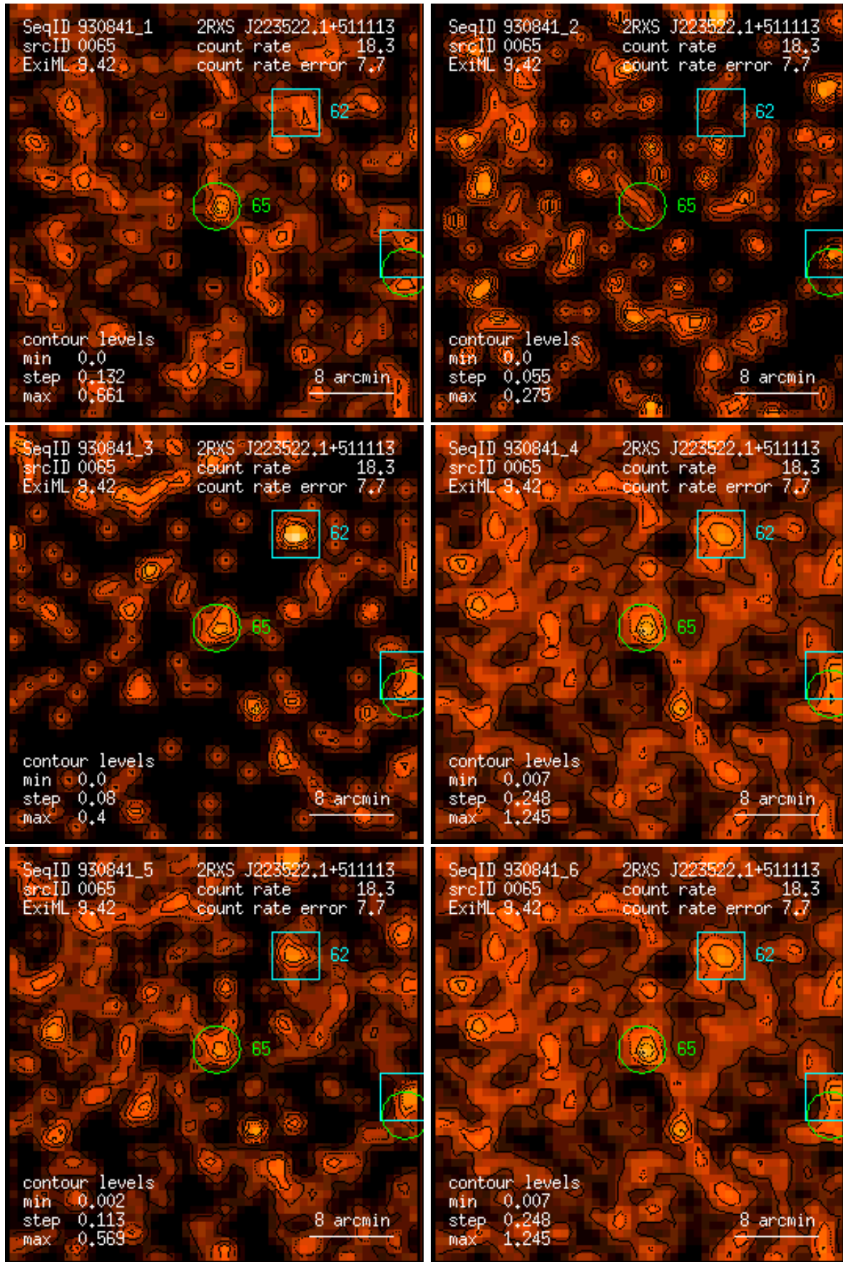
Figure 65: RASS 930841: detection 0065: band rate images, Gaussian filter: (1) PSPC channels 11 – 41, (2) 52 – 90, (3) 91 – 201, (4) 11 – 235, (5) 52 – 201, (6) 11 – 201. Broad band rates in counts/ks. Band rate contour levels in counts/ks/arcmin 2 .
