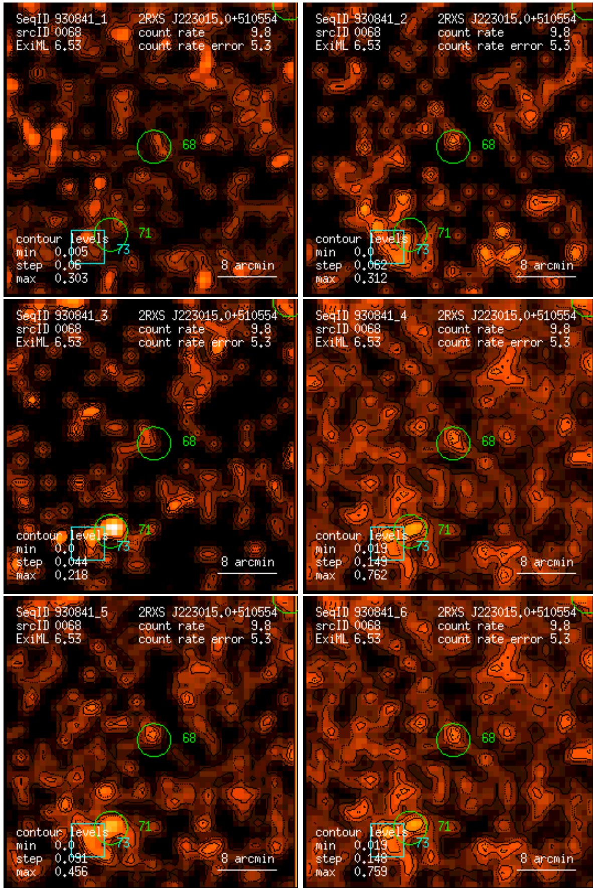
Figure 68: RASS 930841: detection 0068: band rate images, Gaussian filter: (1) PSPC channels 11 – 41, (2) 52 – 90, (3) 91 – 201, (4) 11 – 235, (5) 52 – 201, (6) 11 – 201. Broad band rates in counts/ks. Band rate contour levels in counts/ks/arcmin 2 .
