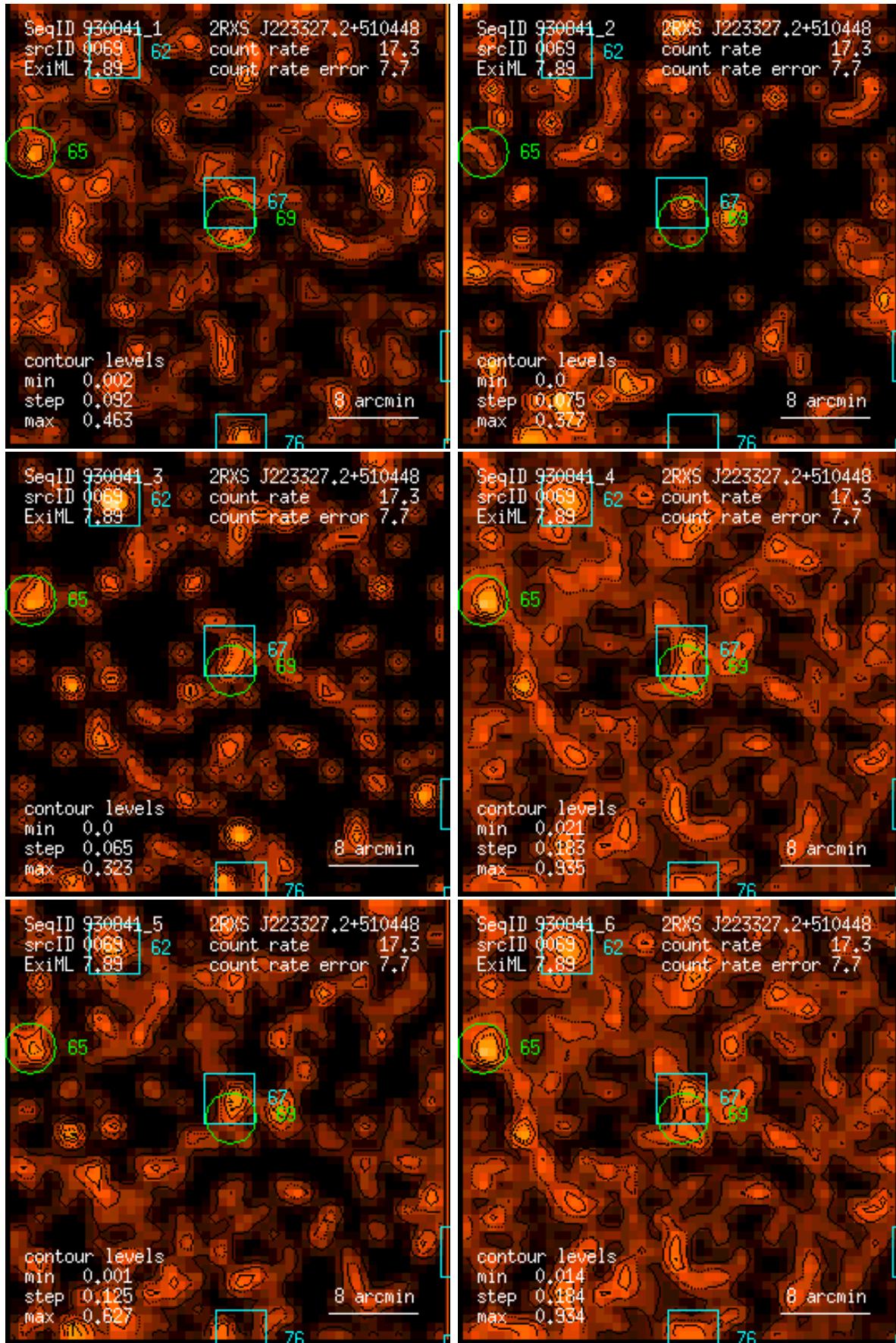
Figure 69: RASS 930841: detection 0069: band rate images, Gaussian filter: (1) PSPC channels 11 – 41, (2) 52 – 90, (3) 91 – 201, (4) 11 – 235, (5) 52 – 201, (6) 11 – 201. Broad band rates in counts/ks. Band rate contour levels in counts/ks/arcmin 2 .
