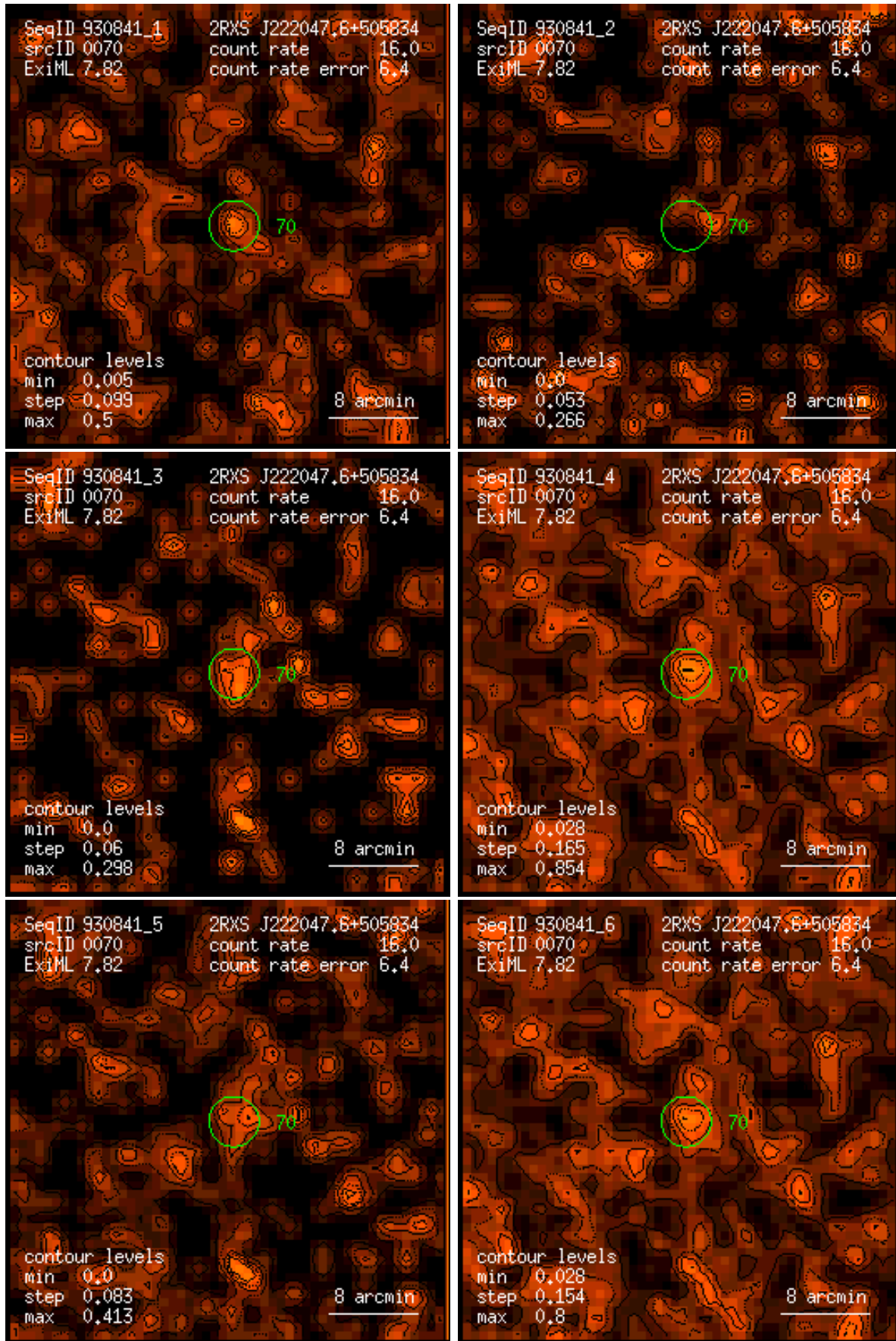
Figure 70: RASS 930841: detection 0070: band rate images, Gaussian filter: (1) PSPC channels 11 – 41, (2) 52 – 90, (3) 91 – 201, (4) 11 – 235, (5) 52 – 201, (6) 11 – 201. Broad band rates in counts/ks. Band rate contour levels in counts/ks/arcmin 2 .
