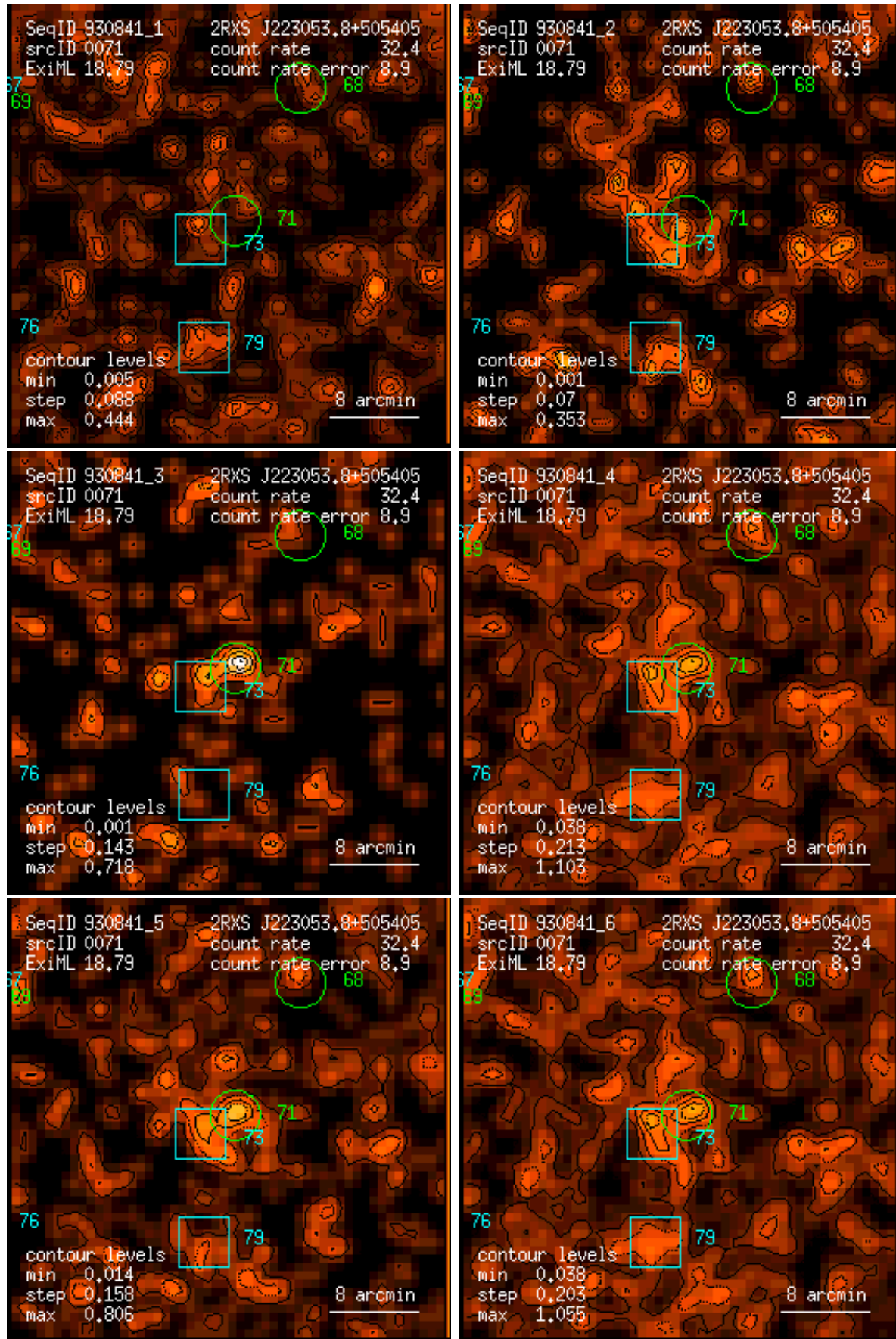
Figure 71: RASS 930841: detection 0071: band rate images, Gaussian filter: (1) PSPC channels 11 – 41, (2) 52 – 90, (3) 91 – 201, (4) 11 – 235, (5) 52 – 201, (6) 11 – 201. Broad band rates in counts/ks. Band rate contour levels in counts/ks/arcmin 2 .
