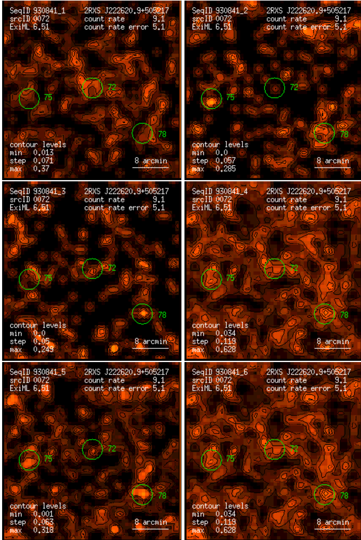
Figure 72: RASS 930841: detection 0072: band rate images, Gaussian filter: (1) PSPC channels 11 – 41, (2) 52 – 90, (3) 91 – 201, (4) 11 – 235, (5) 52 – 201, (6) 11 – 201. Broad band rates in counts/ks. Band rate contour levels in counts/ks/arcmin 2 .
