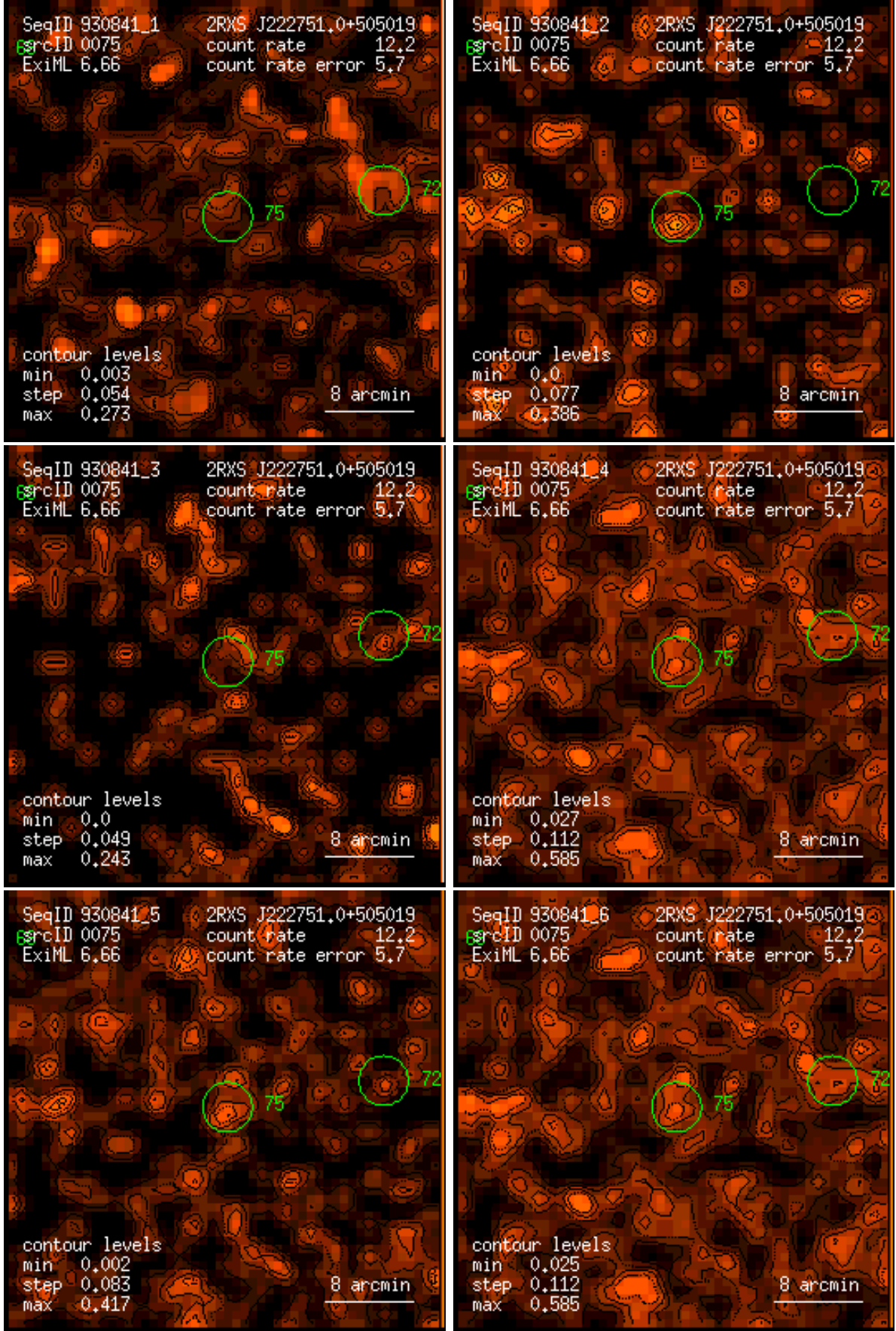
Figure 75: RASS 930841: detection 0075: band rate images, Gaussian filter: (1) PSPC channels 11 – 41, (2) 52 – 90, (3) 91 – 201, (4) 11 – 235, (5) 52 – 201, (6) 11 – 201. Broad band rates in counts/ks. Band rate contour levels in counts/ks/arcmin 2 .
