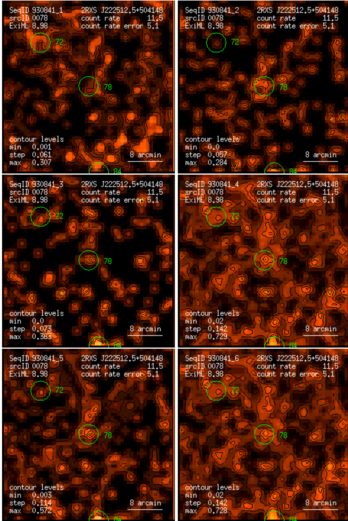
Figure 78: RASS 930841: detection 0078: band rate images, Gaussian filter: (1) PSPC channels 11 – 41, (2) 52 – 90, (3) 91 – 201, (4) 11 – 235, (5) 52 – 201, (6) 11 – 201. Broad band rates in counts/ks. Band rate contour levels in counts/ks/arcmin 2 .
