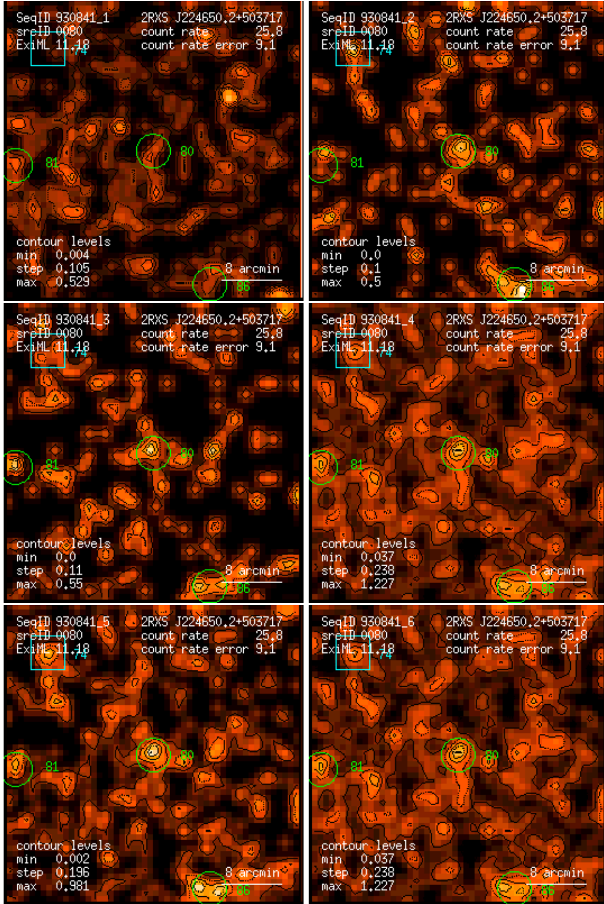
Figure 80: RASS 930841: detection 0080: band rate images, Gaussian filter: (1) PSPC channels 11 – 41, (2) 52 – 90, (3) 91 – 201, (4) 11 – 235, (5) 52 – 201, (6) 11 – 201. Broad band rates in counts/ks. Band rate contour levels in counts/ks/arcmin 2 .
