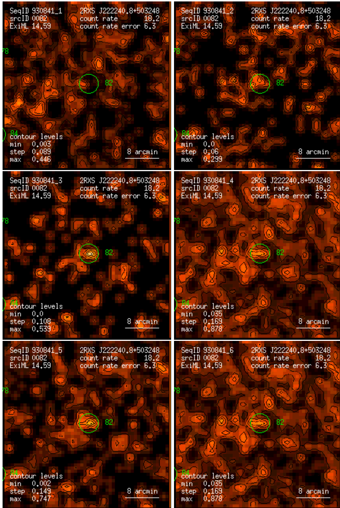
Figure 82: RASS 930841: detection 0082: band rate images, Gaussian filter: (1) PSPC channels 11 – 41, (2) 52 – 90, (3) 91 – 201, (4) 11 – 235, (5) 52 – 201, (6) 11 – 201. Broad band rates in counts/ks. Band rate contour levels in counts/ks/arcmin 2 .
