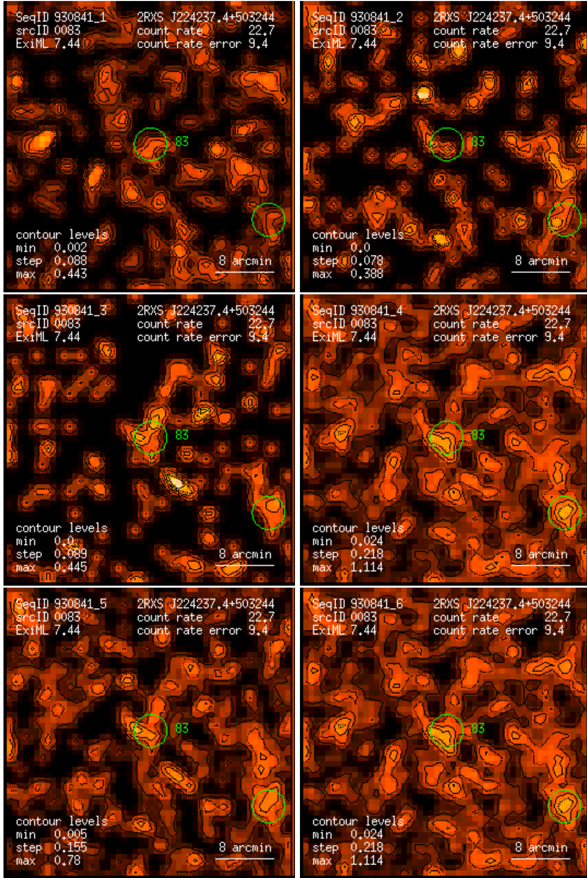
Figure 83: RASS 930841: detection 0083: band rate images, Gaussian filter: (1) PSPC channels 11 – 41, (2) 52 – 90, (3) 91 – 201, (4) 11 – 235, (5) 52 – 201, (6) 11 – 201. Broad band rates in counts/ks. Band rate contour levels in counts/ks/arcmin 2 .
