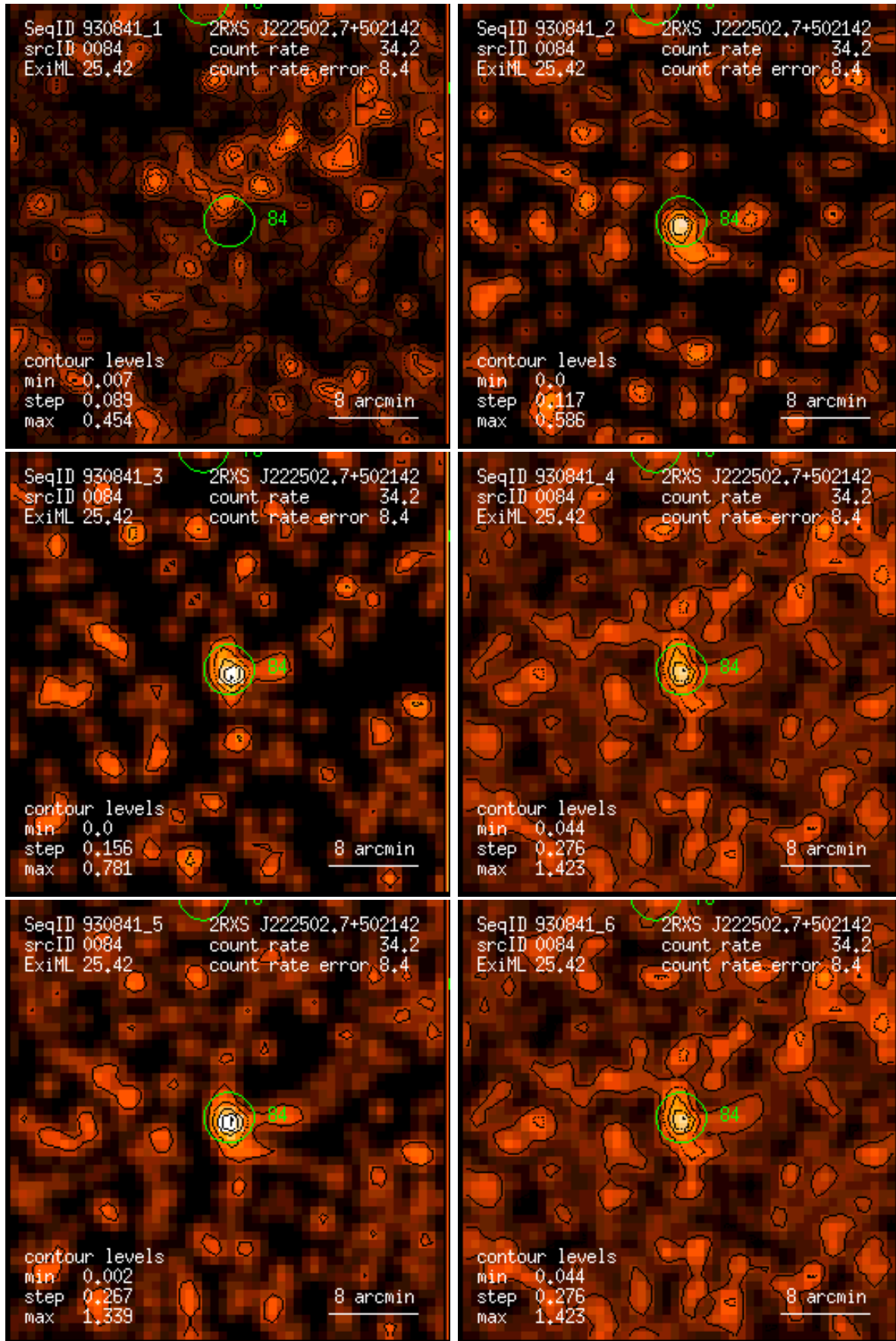
Figure 84: RASS 930841: detection 0084: band rate images, Gaussian filter: (1) PSPC channels 11 – 41, (2) 52 – 90, (3) 91 – 201, (4) 11 – 235, (5) 52 – 201, (6) 11 – 201. Broad band rates in counts/ks. Band rate contour levels in counts/ks/arcmin 2 .
